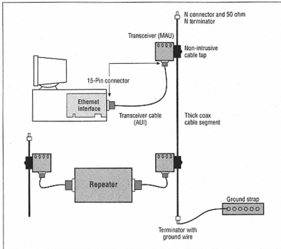
Figure B-3. Connecting a station to a 10BASE5 Ethernet system
