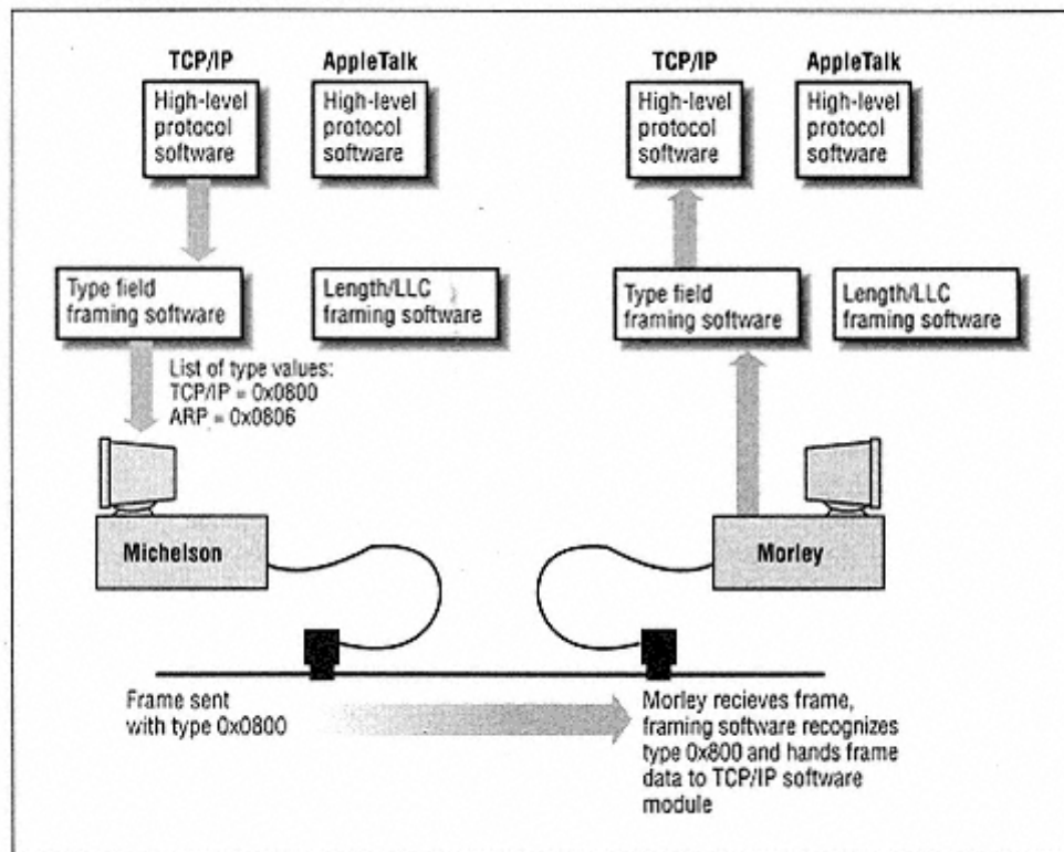
Figure 3-6. Multiplexing high-level protocols
