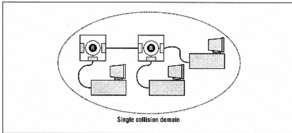
Figure 17-1. Repeater hubs create a single collision domain
