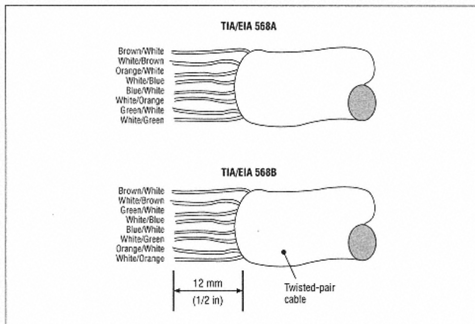
Figure 15-5. Arrange the twisted-pair wires
