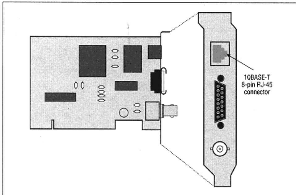
Figure 7-1. 10BASE-T Ethernet interface
