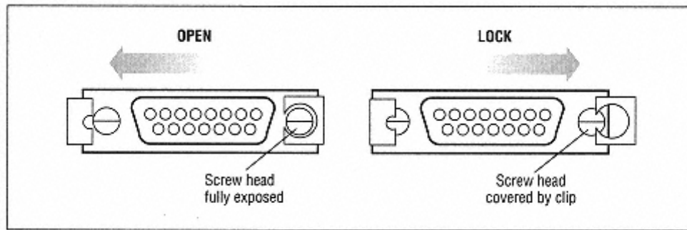
Figure C-1. Sliding latch mechanism
