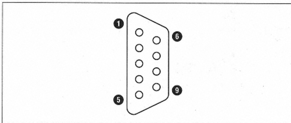
Figure 12-5. 9-pin D-subminiature connector
