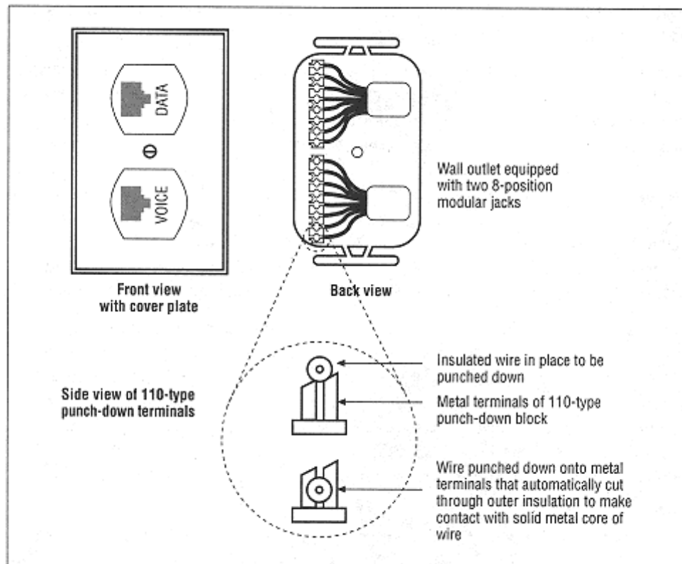
Figure 15-1. Punch-down connector
