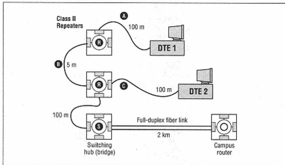
Figure 13-5. One possible maximum 100 Mbps configuration
