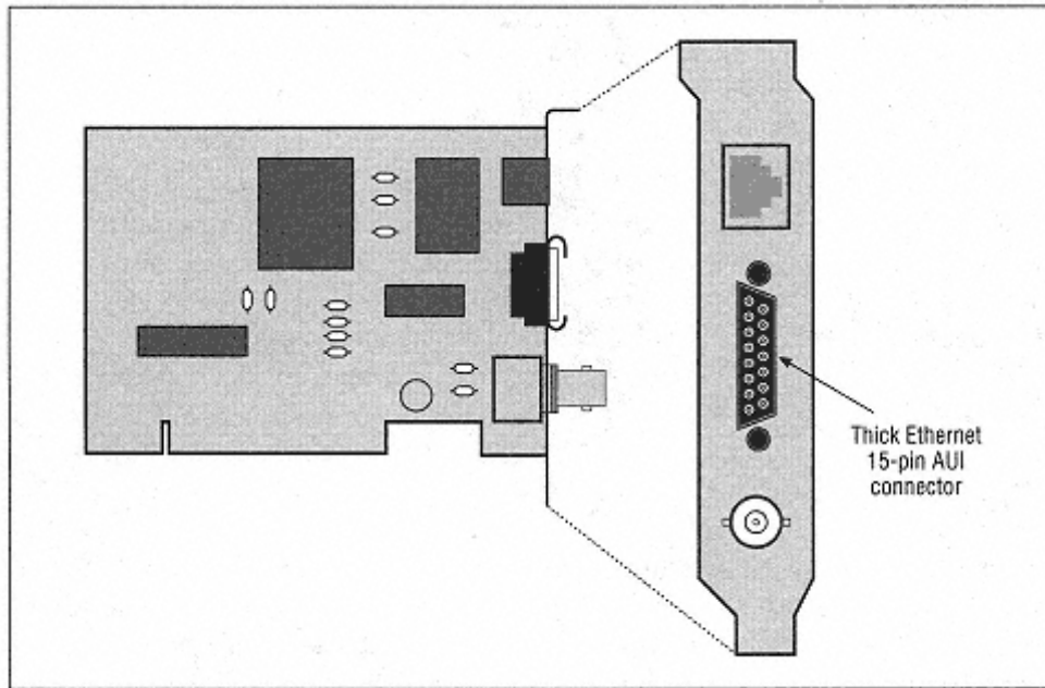
Figure B-1. Thick Ethernet interface
