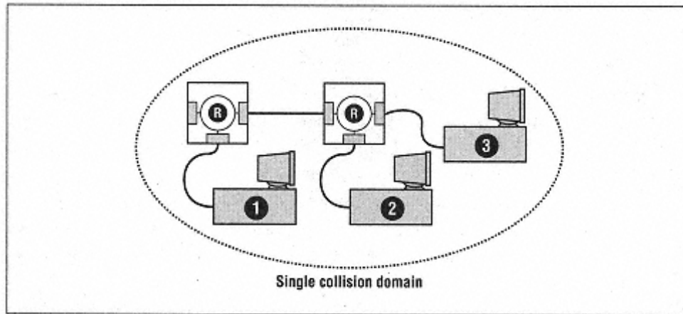
Figure 13-1. Repeater hubs create a single collision domain
