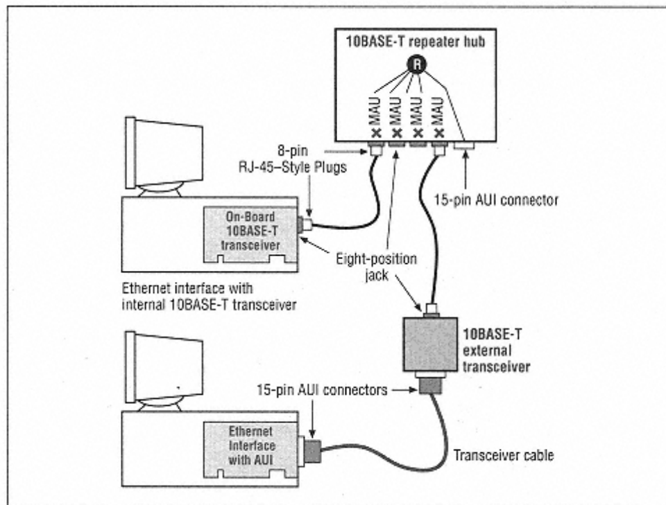
Figure 7-3. Connecting a station to a 10BASE-T Ethernet system
