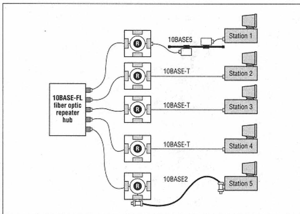
Figure 17-7. Fiber optic backbone
