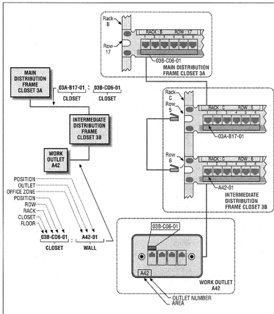
Figure 14-3. Cable administration
