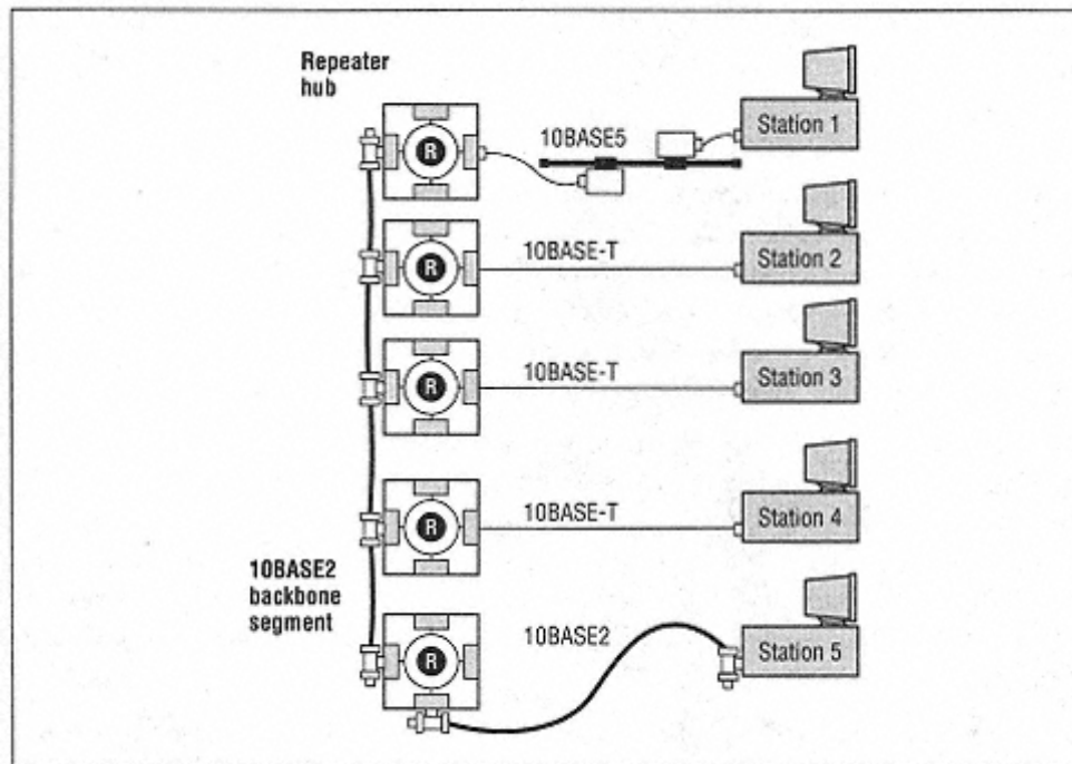
Figure 17-5. Coax backbone
