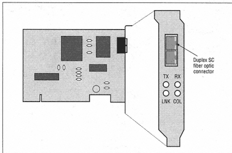
Figure 10-1. 100BASE-FX Ethernet interface
