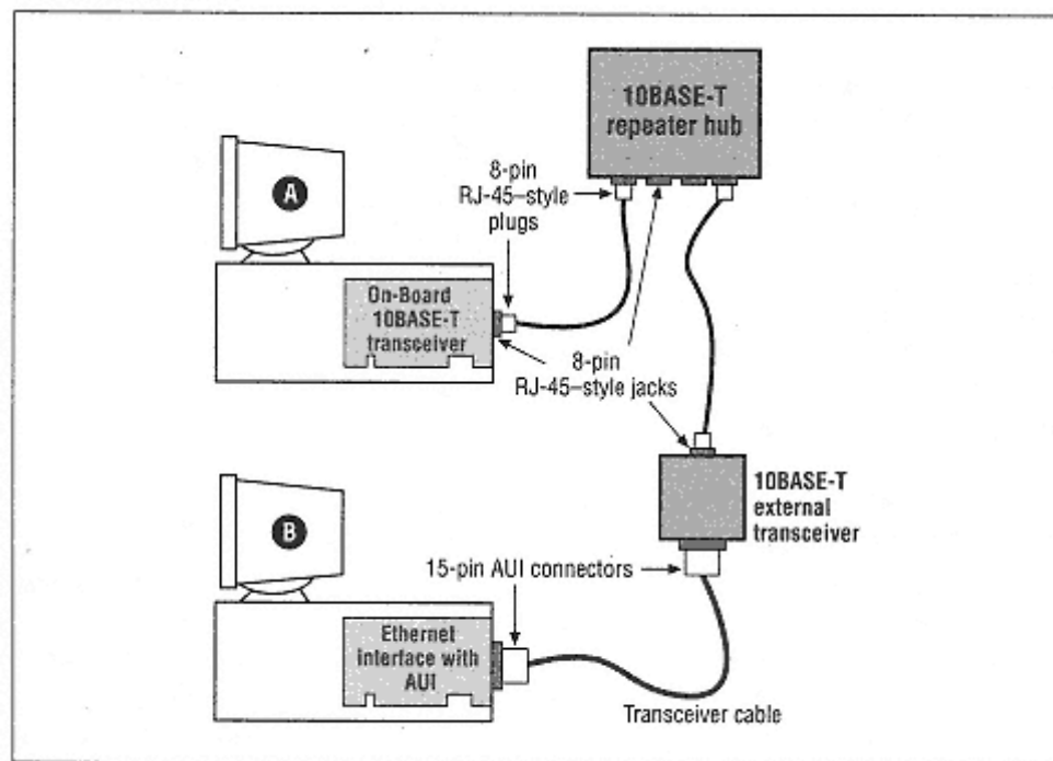
Figure 2-2. A sample 10BASE-T Ethernet connection
