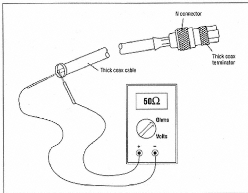
Figure B-35. Testing coaxial segment terminating resistance
