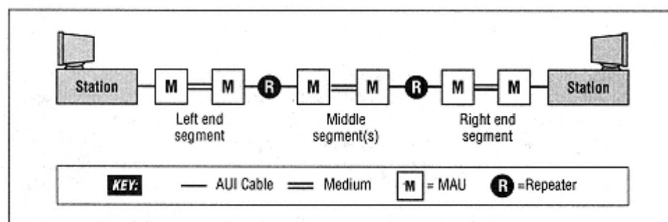
Figure 13-3. Network model for round-trip timing
