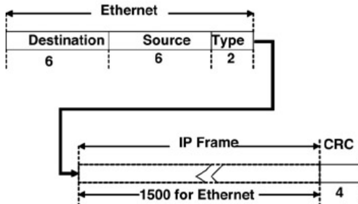
Figure 3.3: Ethernet framing.
