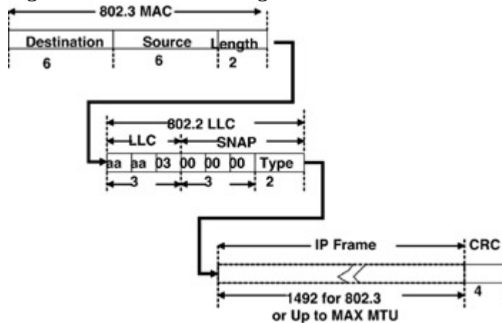
Figure 3.4: 802.3 framing.
