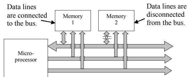
Figure 3. Block diagram of two memory devices sharing a bus
