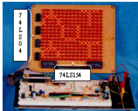
Figure 4. LED matrix display (Project 3)
