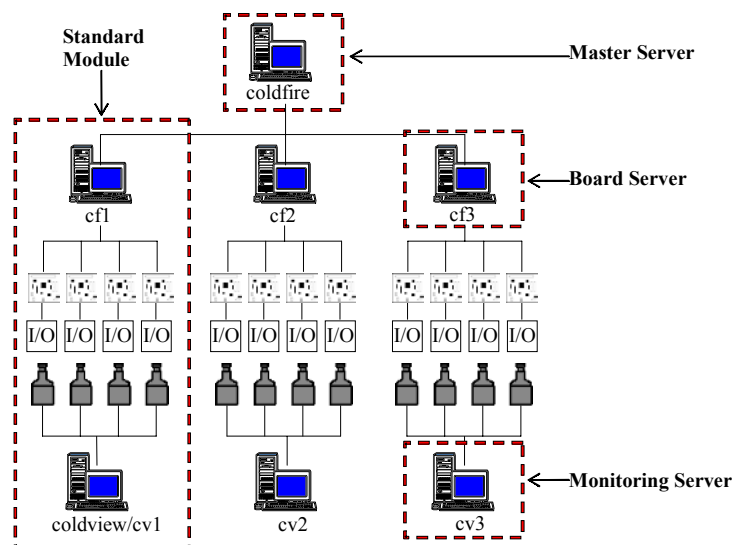
Figure 3. Remotely accessible embedded systems laboratory topology
