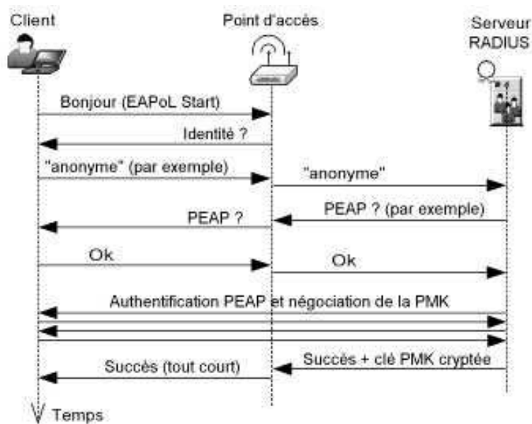
Figure 9.4 — L'authentification 802.1x.
