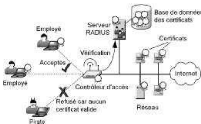
Figure 8.8 — L'authentification EAP/TLS.
