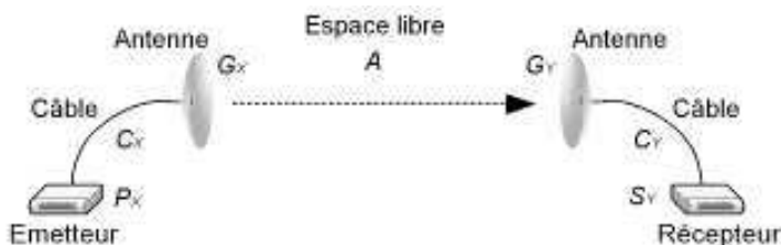
Figure 5.1 — Le bilan radio.
