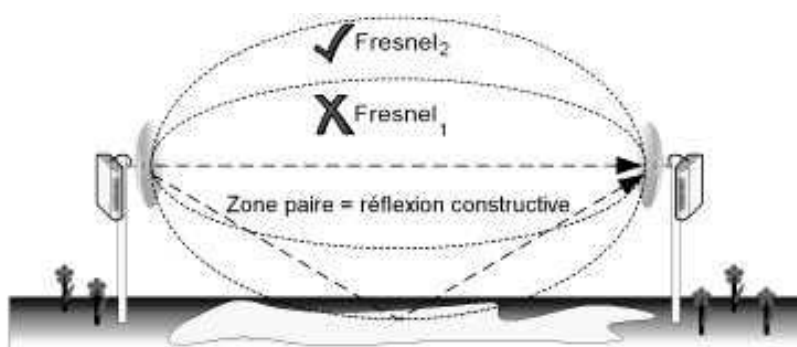
Figure 5.13 — Réflexions constructives ou destructives.
