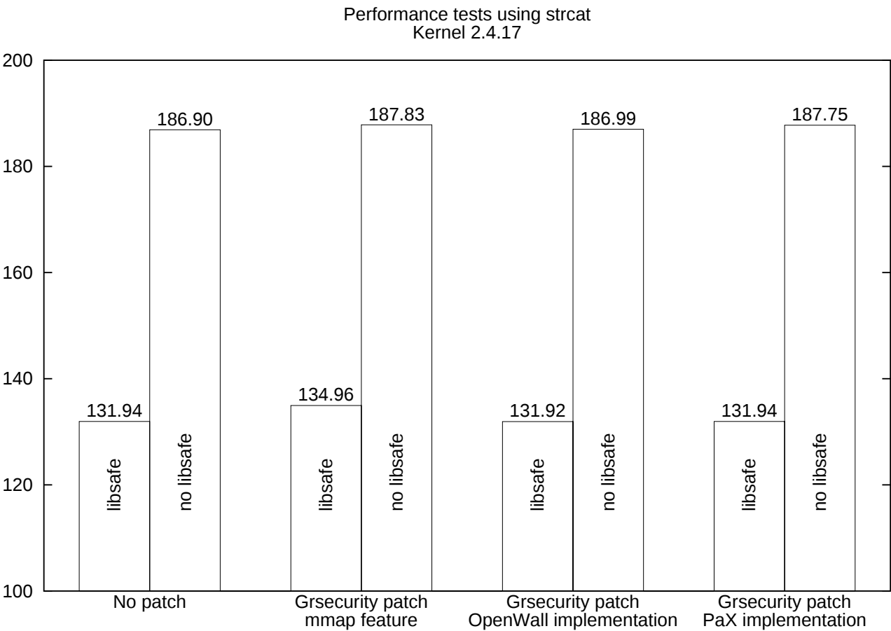
Figure C.1: Performance tests - 1
