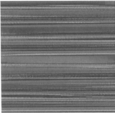
(c) 4 iterations
