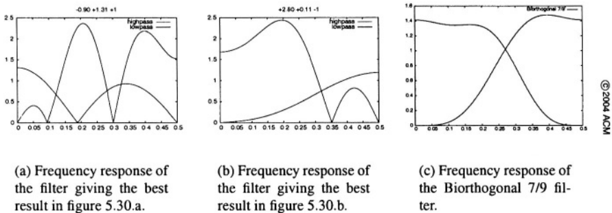
Figure 5.31. Frequency response
