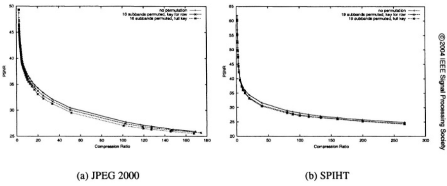
Figure 5.20. Compression performance, Lena image 512 x 512 pixels
