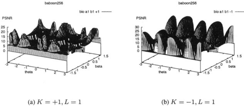
Figure 5.30. Parameterised biorthogonal 4/8 filters.
