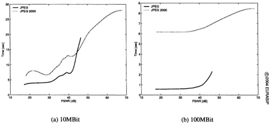
Figure 4.6. Wired connections (ethernet), AES encryption
