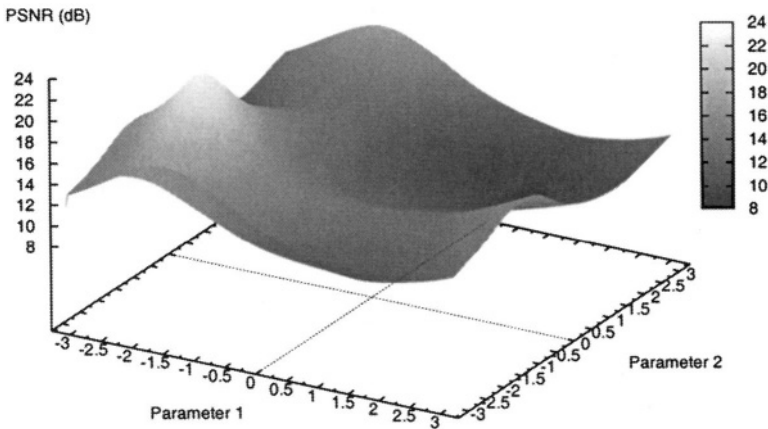
Figure 5.27. Attack against a 2-D parameter scheme, JPEG 2000 compression at ratio 1:10
