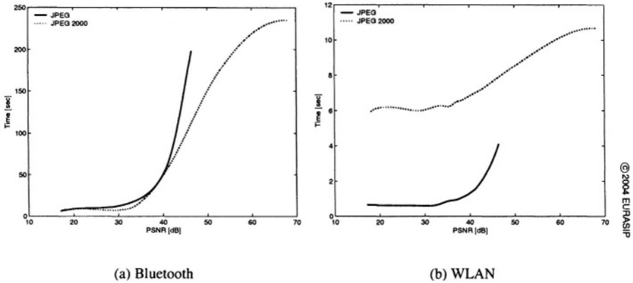
Figure 4.5. Wireless connections, AES encryption.
