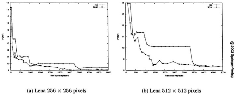
Figure 5.37. Comparison of selective encryption (PSNR of reconstructed images) using resolution or layer progressive encoding - part 2.
