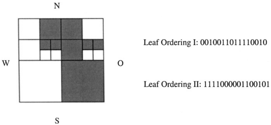
Figure 5.53. Example for leaf ordering I and II.
