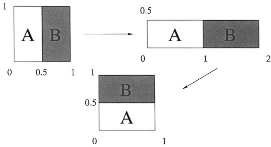
Figure 5.45. Baker Map (1/2,1/2).
