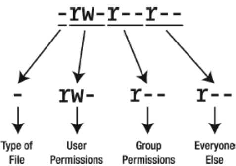
Figure 21-4. The file permissions part of a file listing can be broken down into four separate parts.
