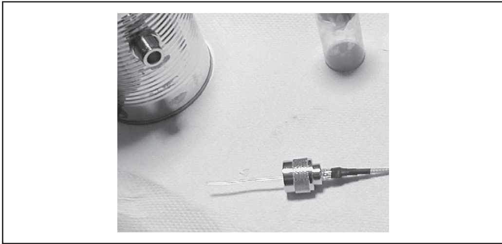
Figure 8-9 Antenna wire unbroken and extended for passing through the shielded connector into the cantenna body (photo courtesy of Julian “HammerJammer” Ho)
