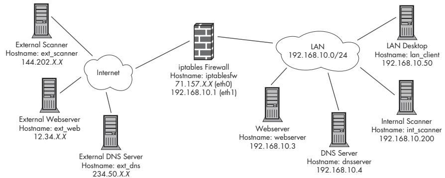
Figure 8-1: Default network diagram
