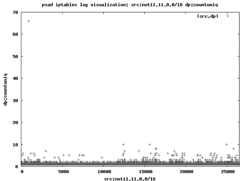
Figure 14-3: Source IP addresses vs. number of unique ports
