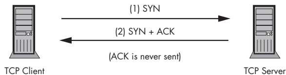
Figure 3-5: TCP half-open scan
