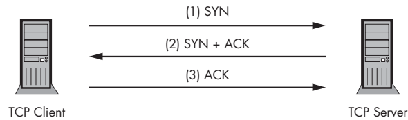
Figure 3-4: TCP three-way handshake
