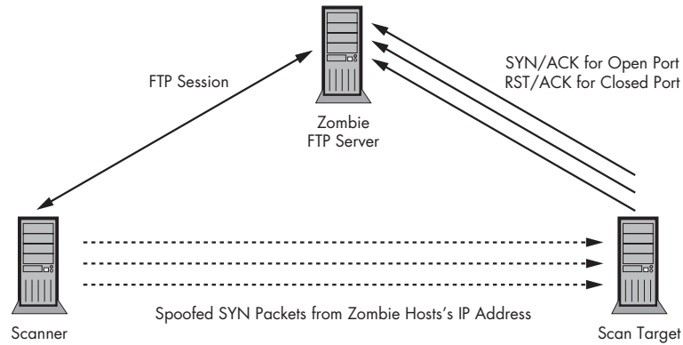
Figure 3-6: TCP idle scan
