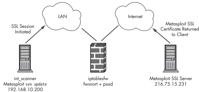
Figure 11-1: Metasploit update through fwsnort and psad
