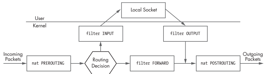
Figure 1-1: iptables packet flow
