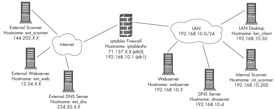
Figure 3-2: Default network diagram
