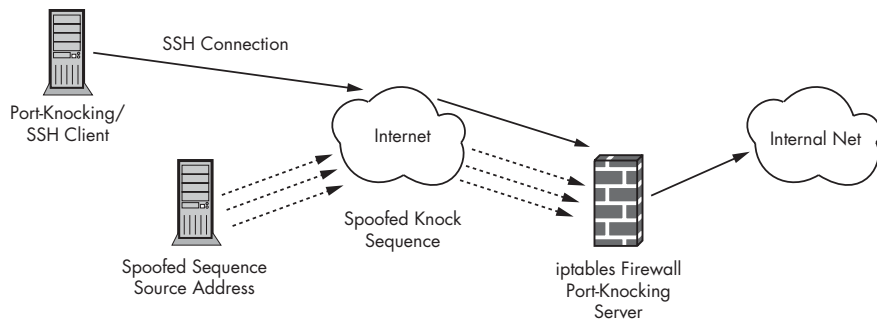
Figure 12-1: A port-knocking network
