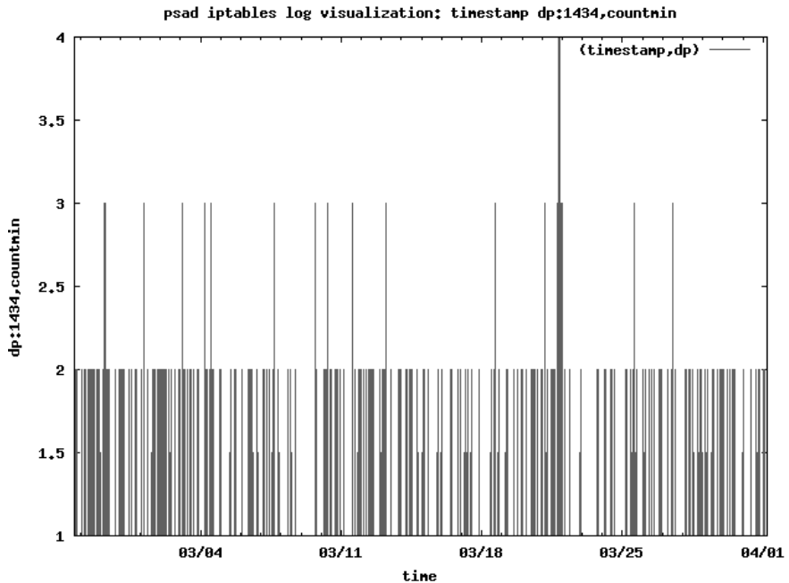
Figure 14-10: Slammer worm packet counts by the minute
