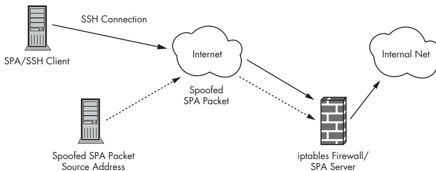
Figure 12-3: An SPA network
