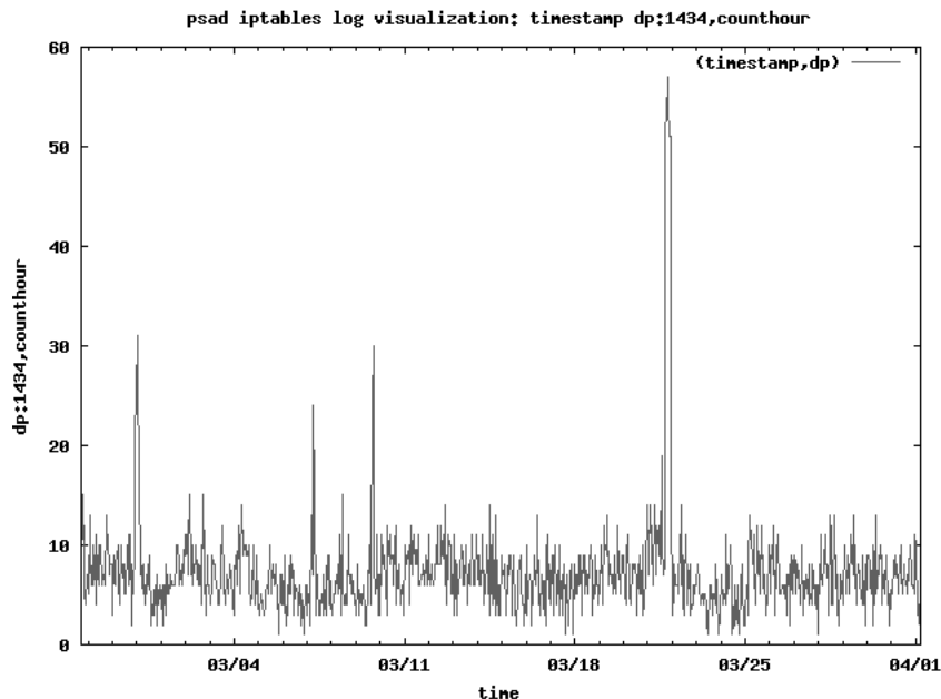
Figure 14-9: Slammer worm packet counts by the hour
