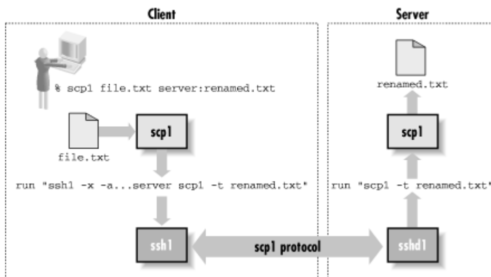
Figure 3.6. scp1 operation
