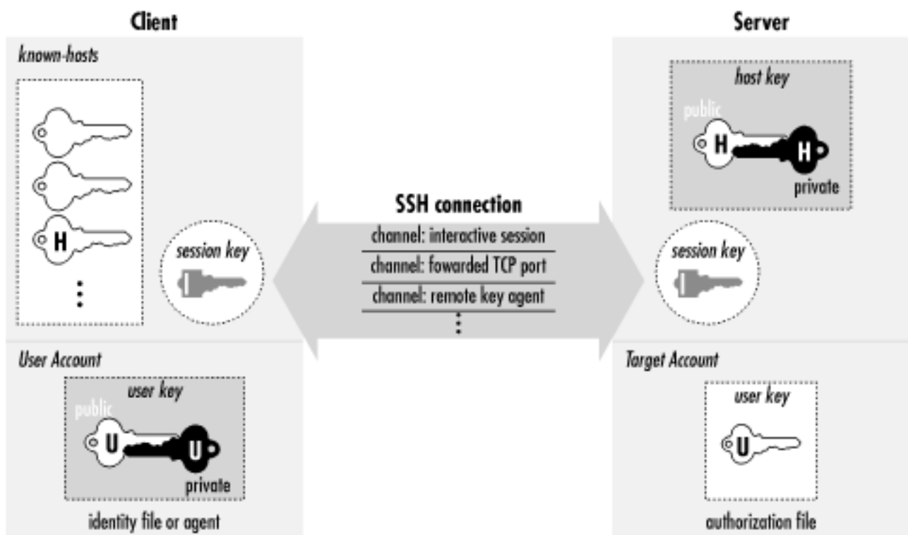
Figure 3.1. SSH architecture
