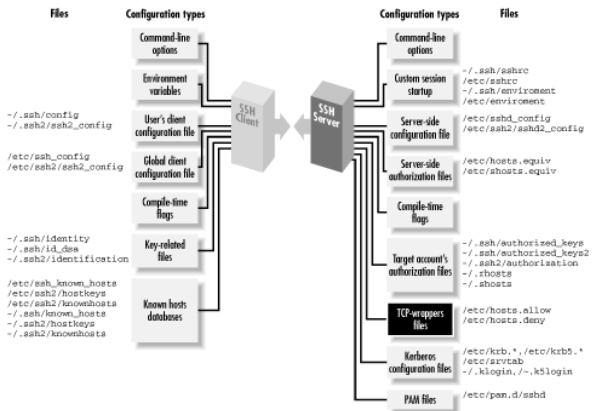
Figure 9.12. TCP-wrappers and SSH configuration (highlighted parts)
