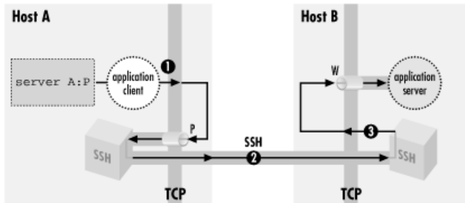
Figure 9.5. A forwarded connection
