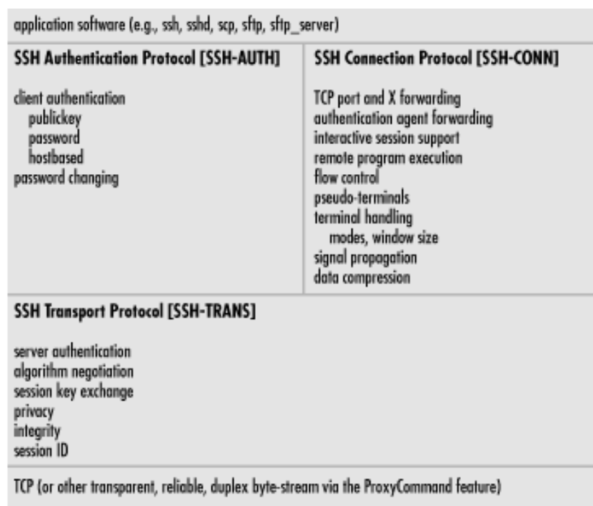
Figure 3.5. SSH-2 protocol family
