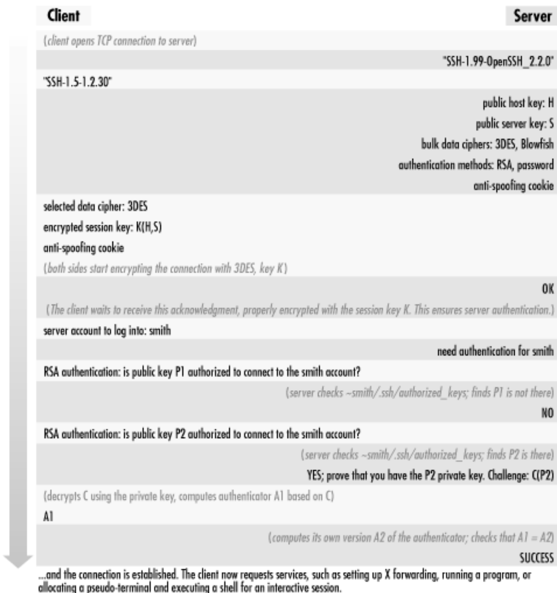
Figure 3.3. SSH-1 protocol exchange
