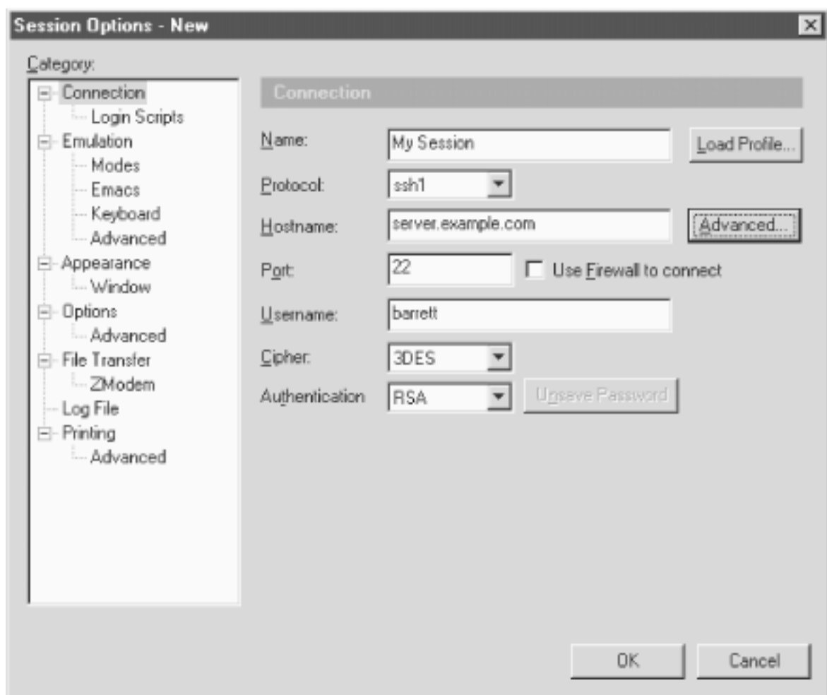
Figure 15.1. Secure CRT Session Options window
