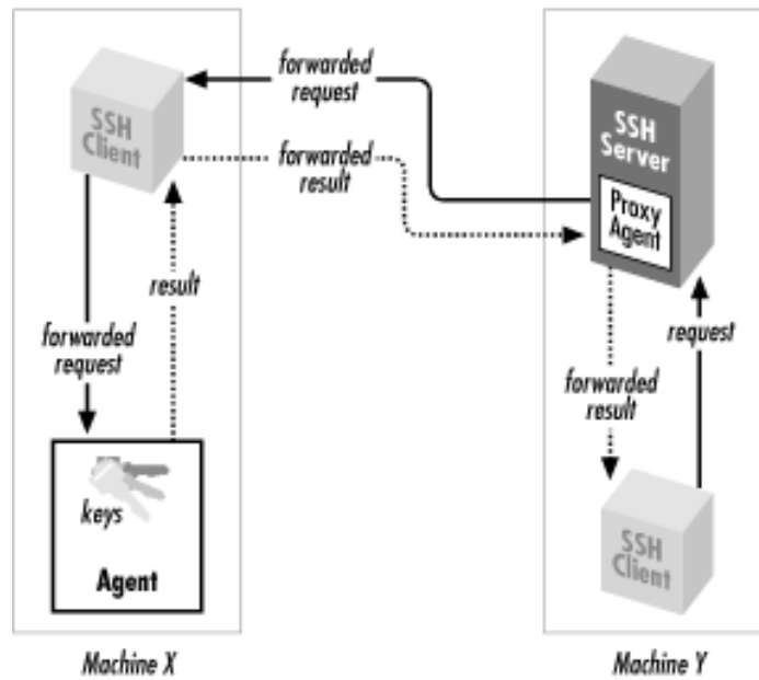
Figure 2.4. How agent forwarding works
