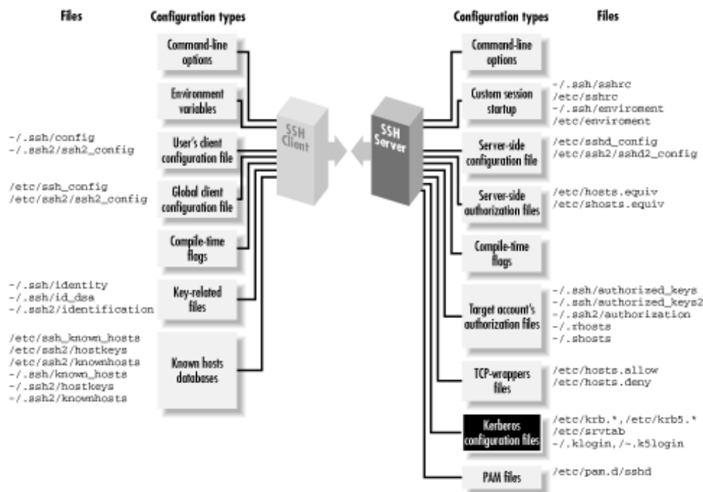
Figure 11.11. Kerberos configuration (highlighted parts)
