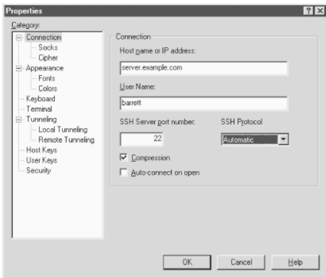
Figure 16.1. F-Secure SSH Client Connection properties window
