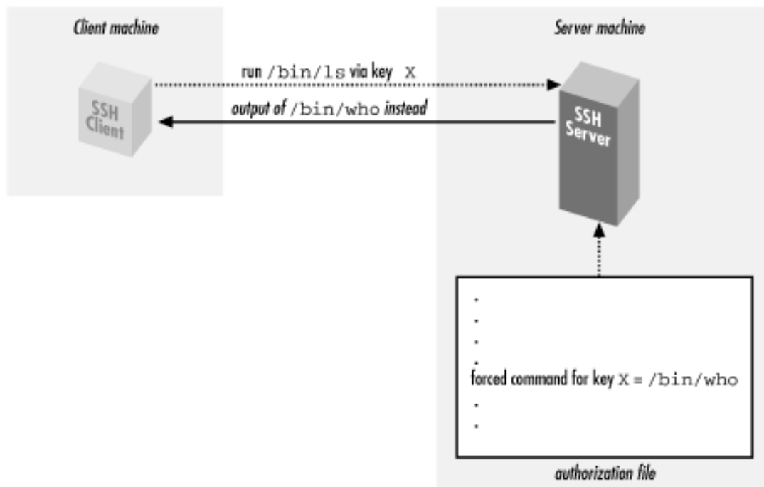
Figure 8.2. Forced command substituting /bin/who for /bin/ls
