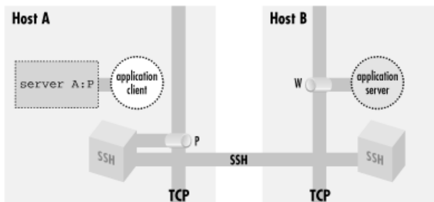
Figure 9.4. A forwarded port
