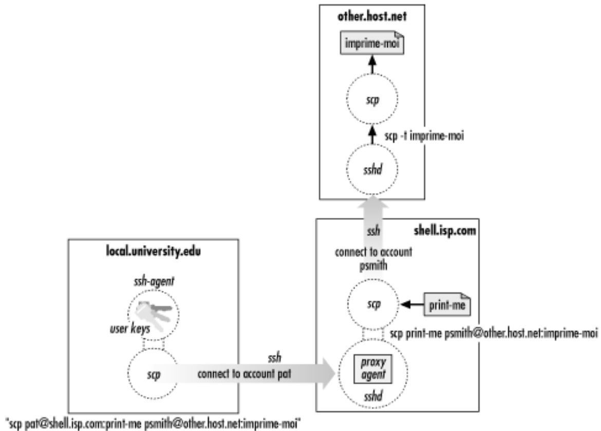
Figure 2.5. Third-party scp with agent forwarding
