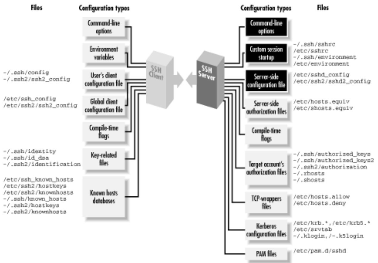
Figure 5.1. Serverwide configuration (highlighted parts)
