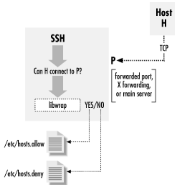
Figure 9.13. TCP-wrapper (libwrap) operation
