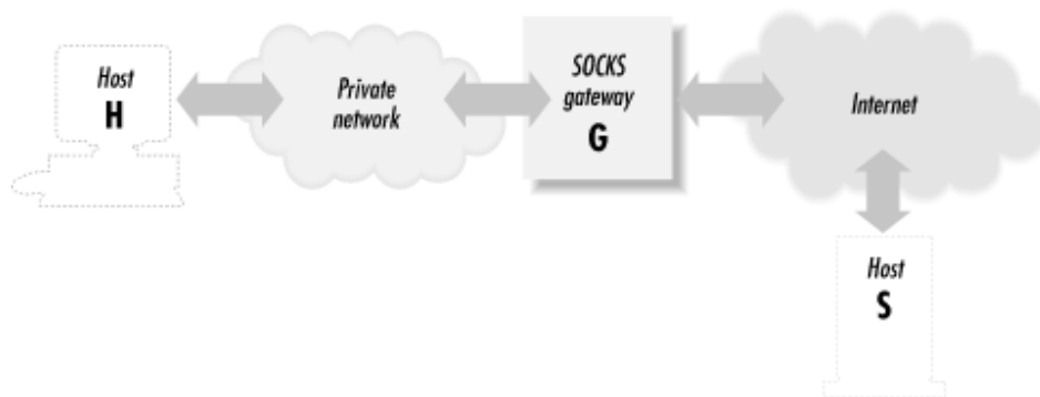
Figure 7.3. A typical SOCKS installation
