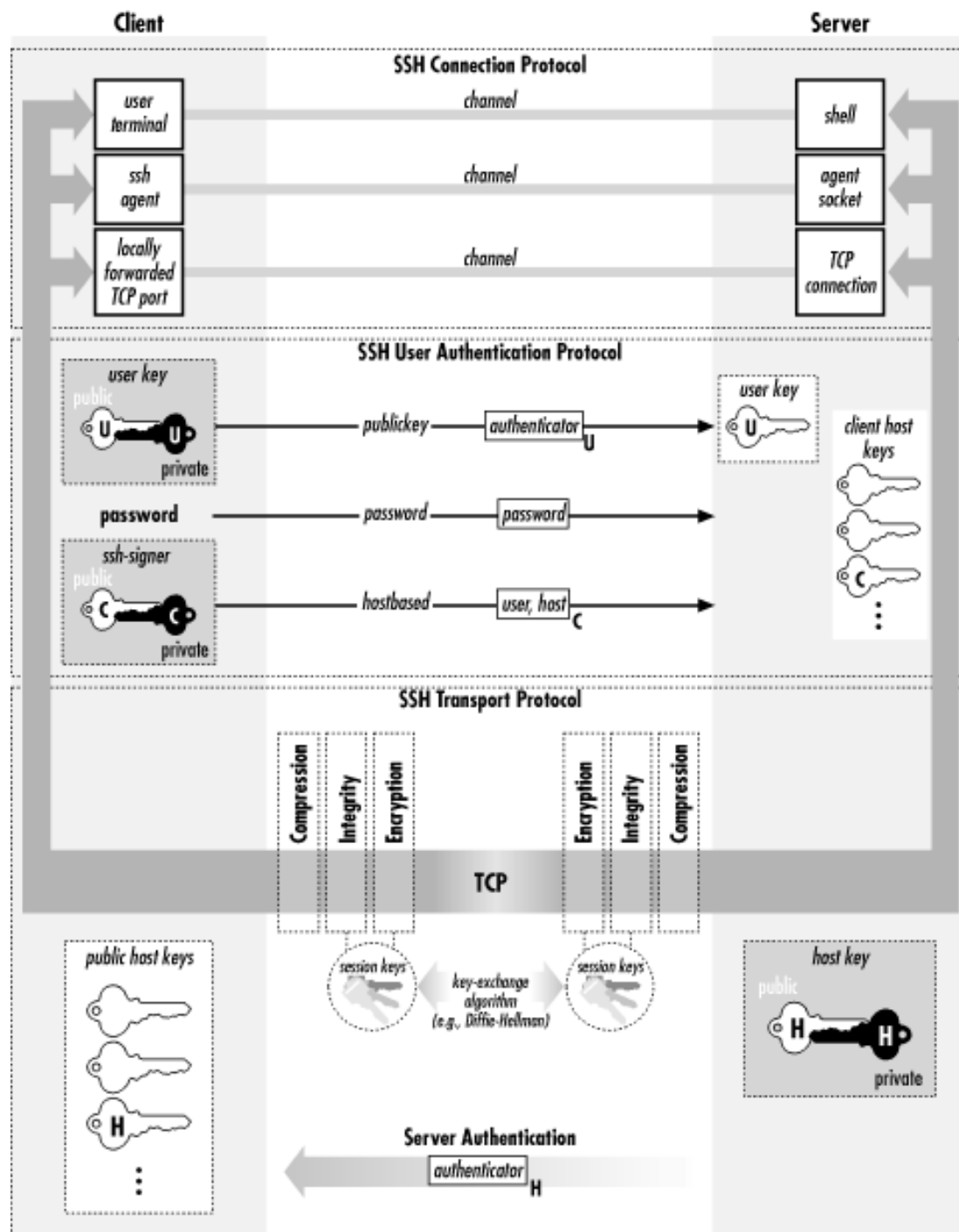
Figure 3.4. SSH-2 architecture
