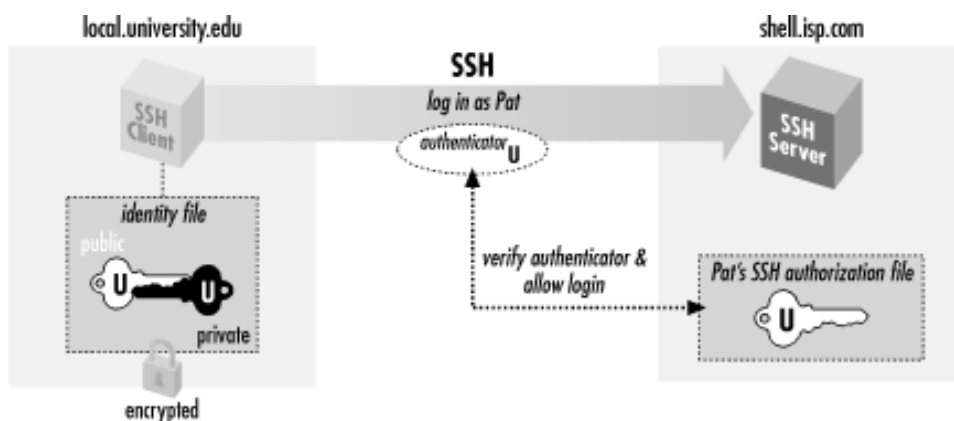
Figure 2.2. Public-key authentication
