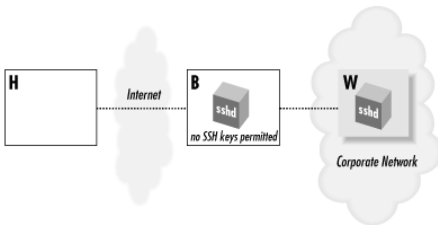
Figure 6.5. Bastion host scenario
