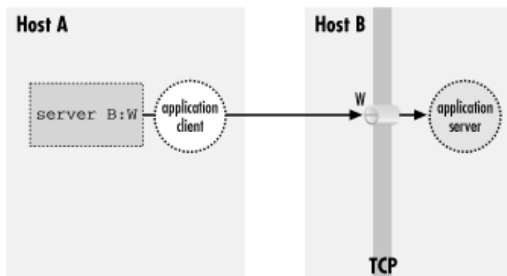
Figure 9.3. Direct client/server connection (no forwarding)
