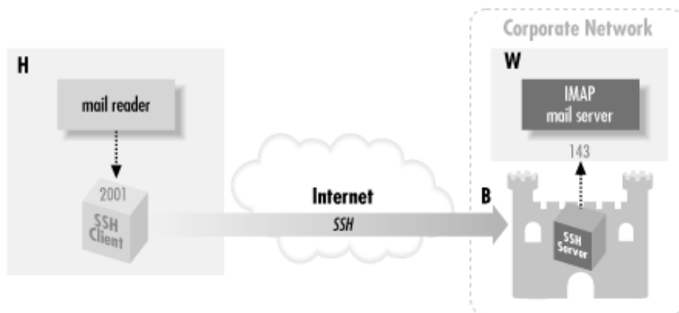
Figure 9.9. Port forwarding through a firewall
