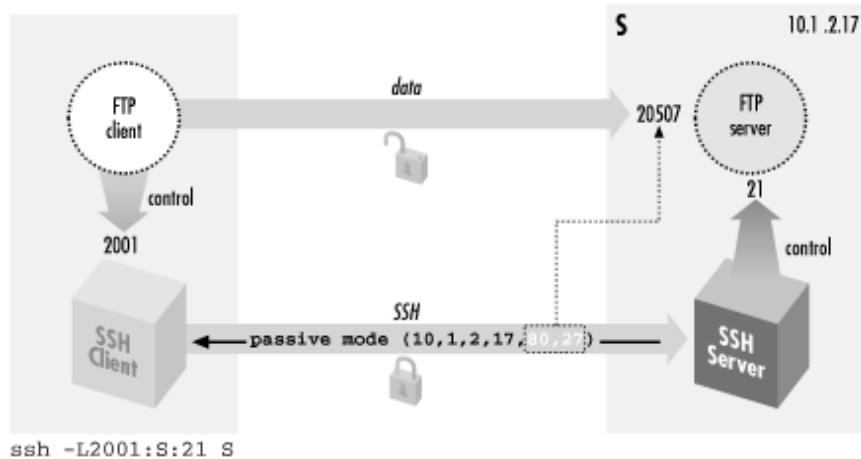
Figure 11.2. Forwarding the control connection
