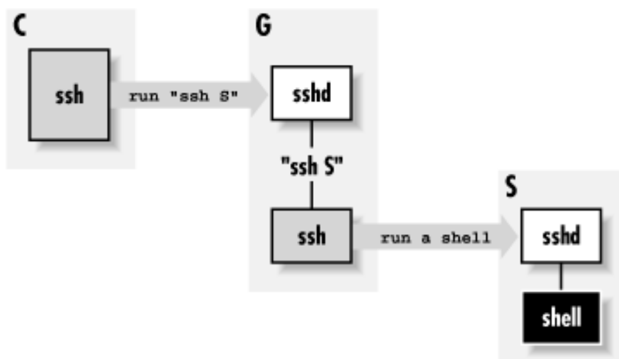
Figure 11.15. Chained SSH connections through a proxy gateway
