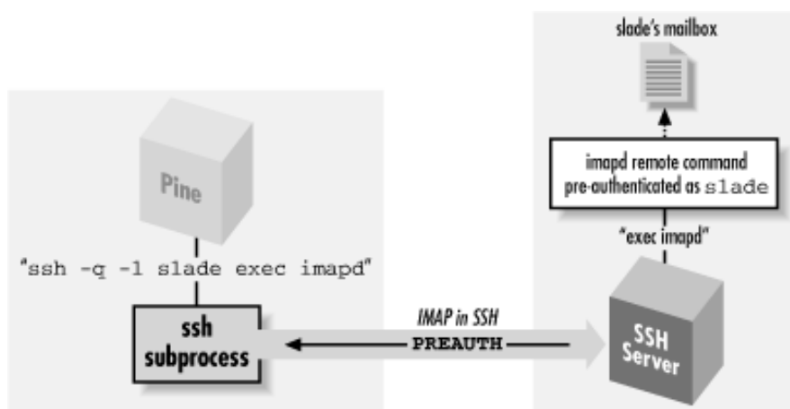
Figure 11.10. Pine/IMAP over SSH, preauthenticated
