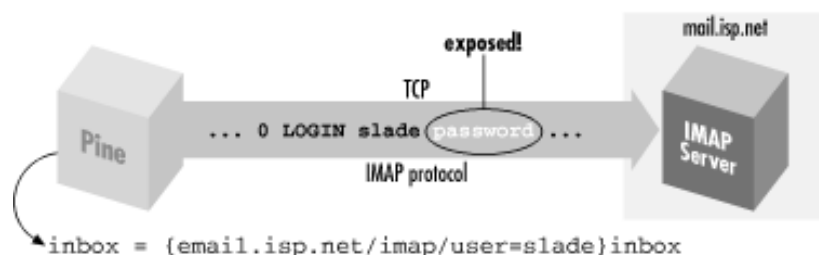
Figure 11.8. A normal IMAP connection
