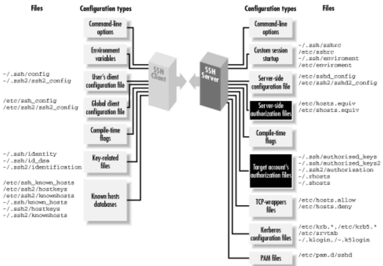
Figure 8.1. Per-account configuration (highlighted parts)
