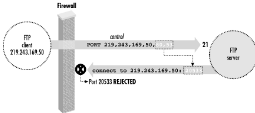
Figure 11.4. FTP client behind a firewall
