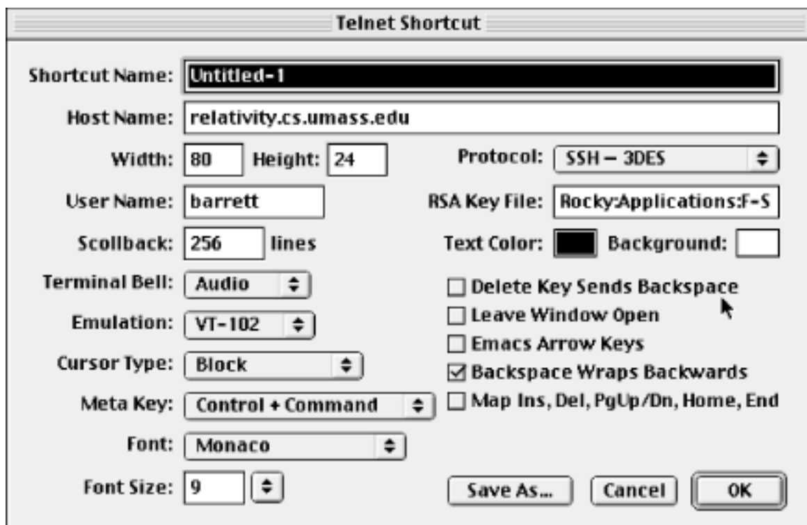
Figure 17.2. NiftyTelnet SSH Settings window
