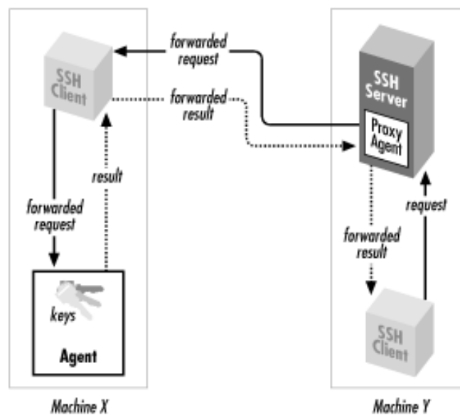
Figure 6.7. How agent forwarding works
