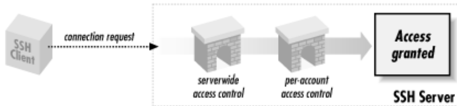
Figure 5.2. Access control levels
