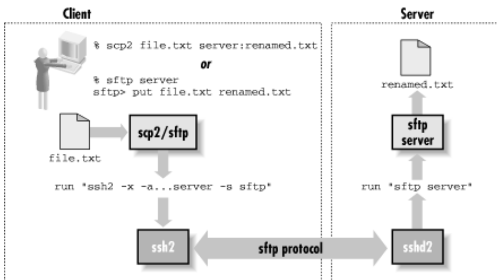
Figure 3.7. scp2/sftp operation
