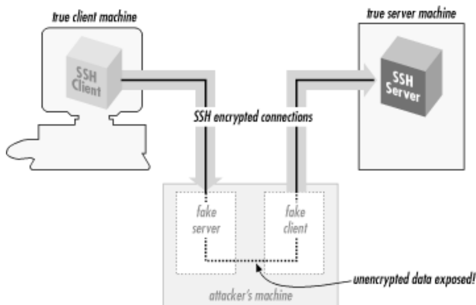
Figure 3.8. Man-in-the-middle attack
