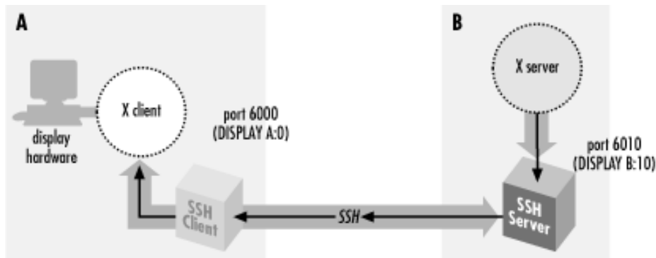
Figure 9.10. X forwarding
