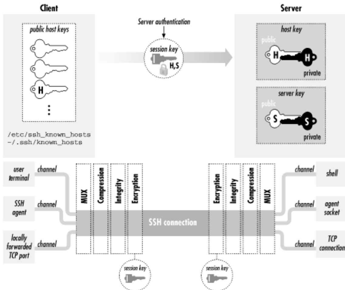
Figure 3.2. SSH-1 architecture
