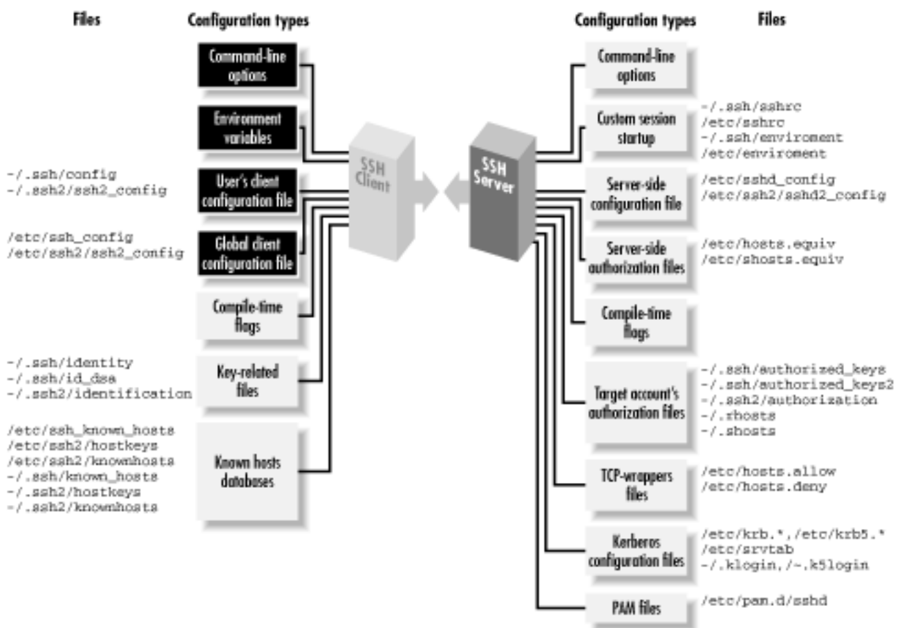
Figure 7.1. Client configuration (highlighted parts)
