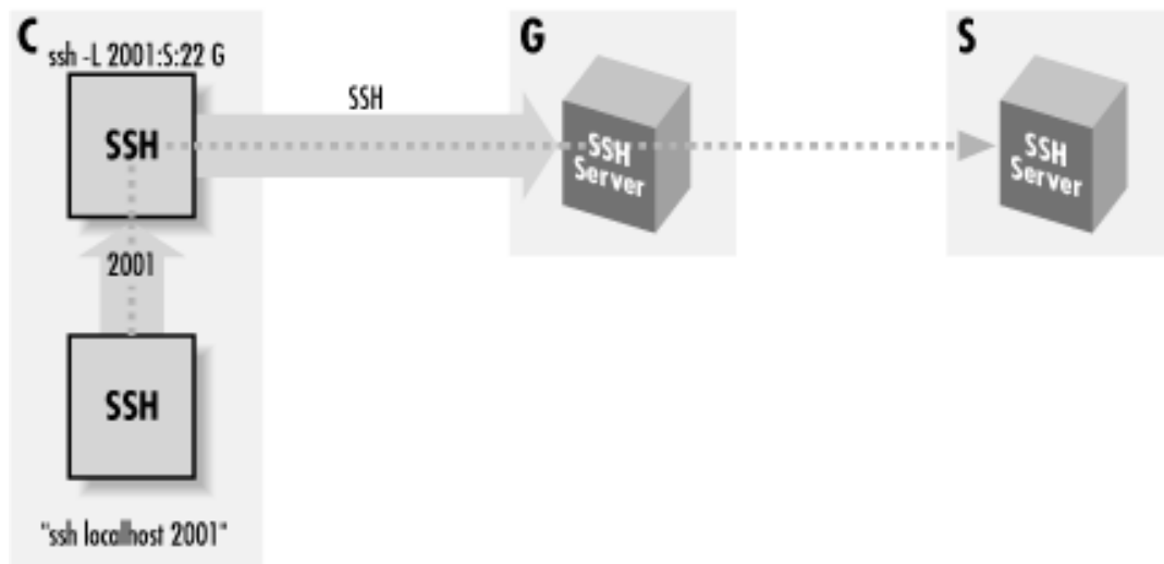
Figure 11.16. Forwarded SSH connection through a proxy gateway
