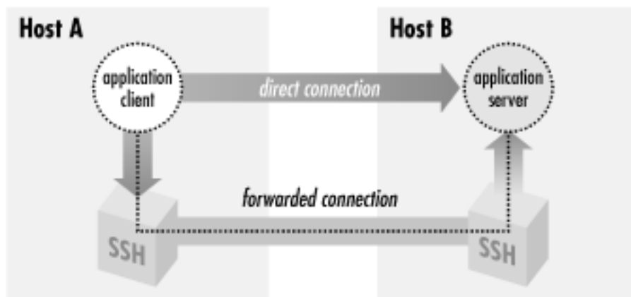
Figure 9.1. SSH forwarding
