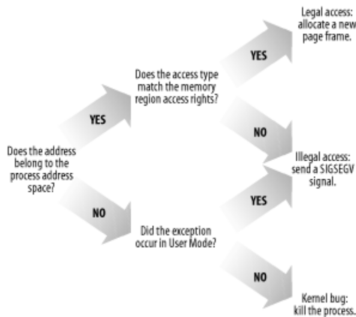
Figure 8-4. Overall scheme for the Page Fault handler
