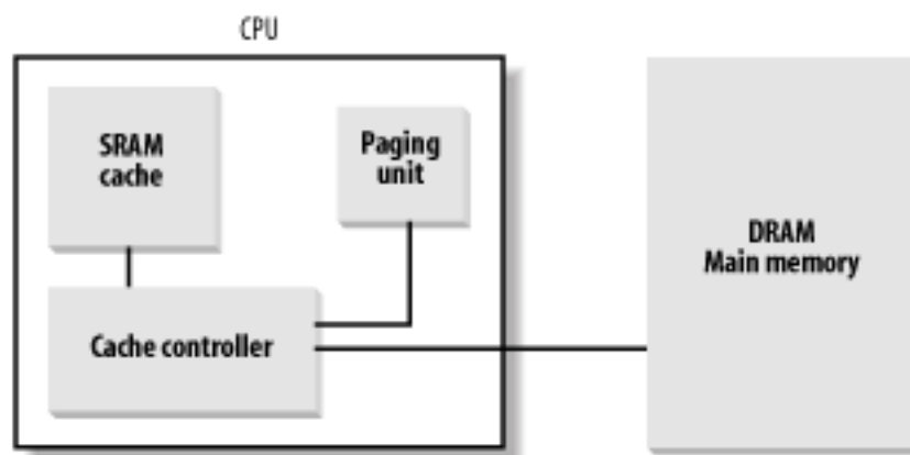
Figure 2-9. Processor hardware cache
