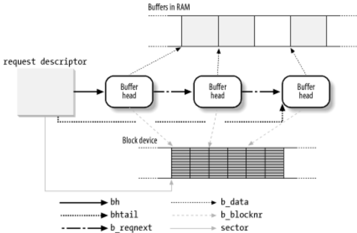
Figure 13-3. A request descriptor and its buffers and sectors
