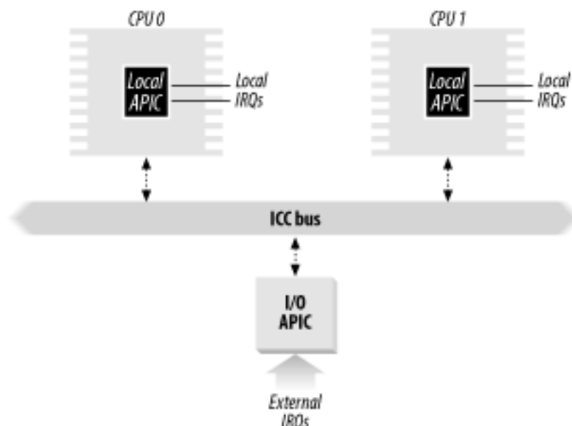
Figure 4-1. Multi-APIC system
