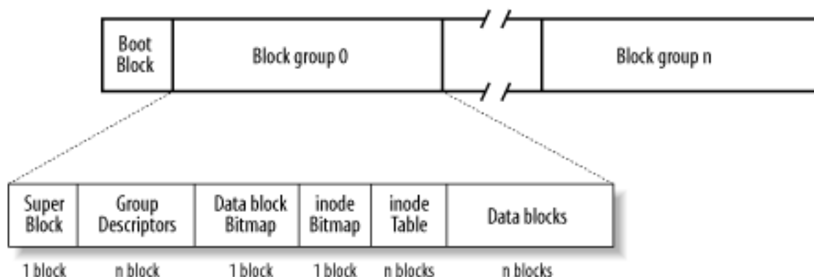
Figure 17-1. Layouts of an Ext2 partition and of an Ext2 block group
