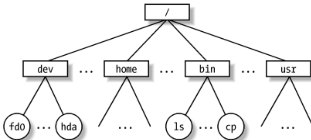
Figure 1-2. An example of a directory tree
