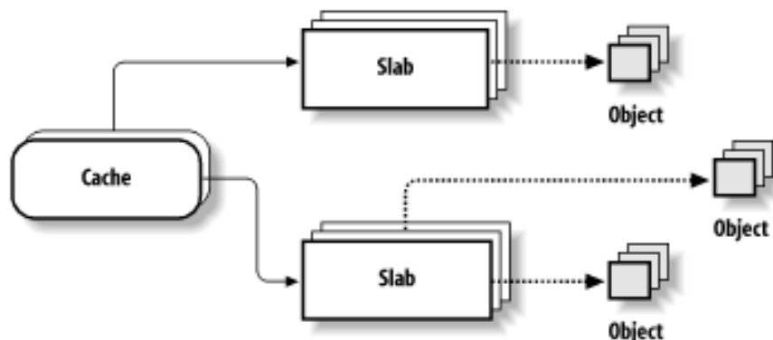
Figure 7-3. The slab allocator components
