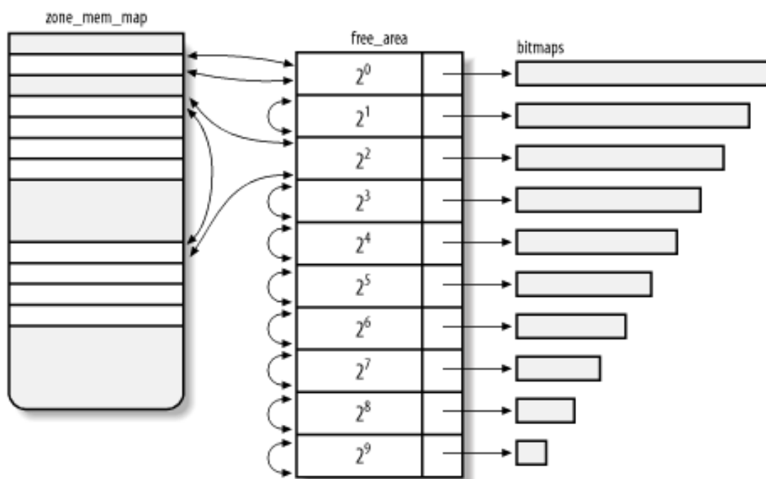
Figure 7-2. Data structures used by the buddy system
