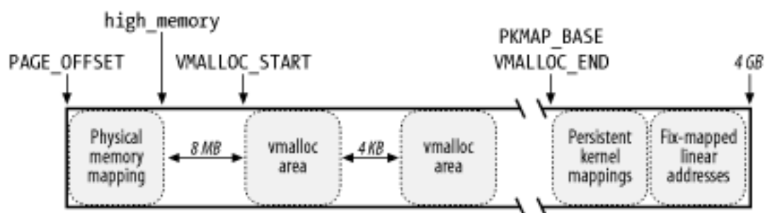
Figure 7-7. The linear address interval starting from PAGE_OFFSET
