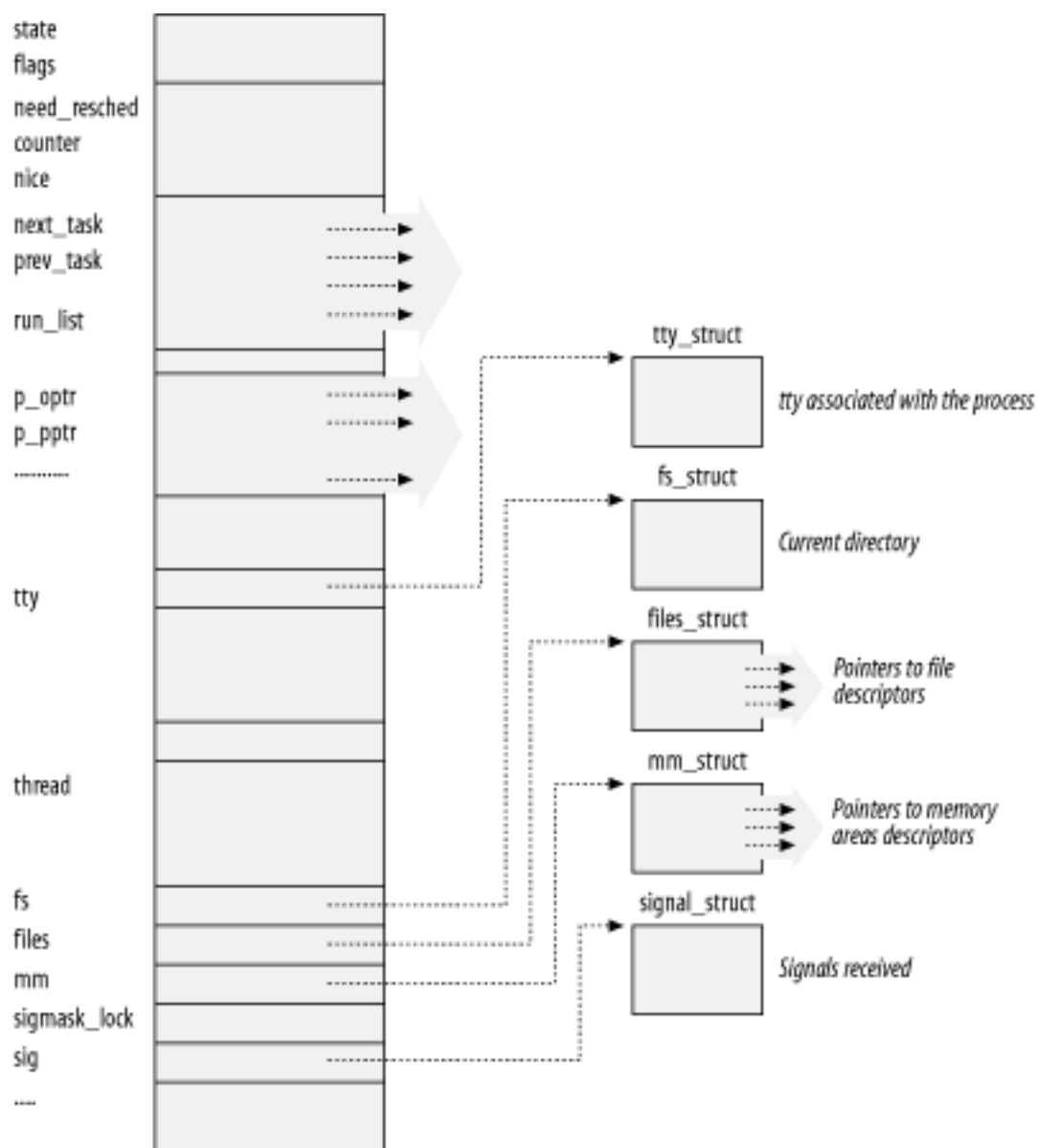
Figure 3-1. The Linux process descriptor
