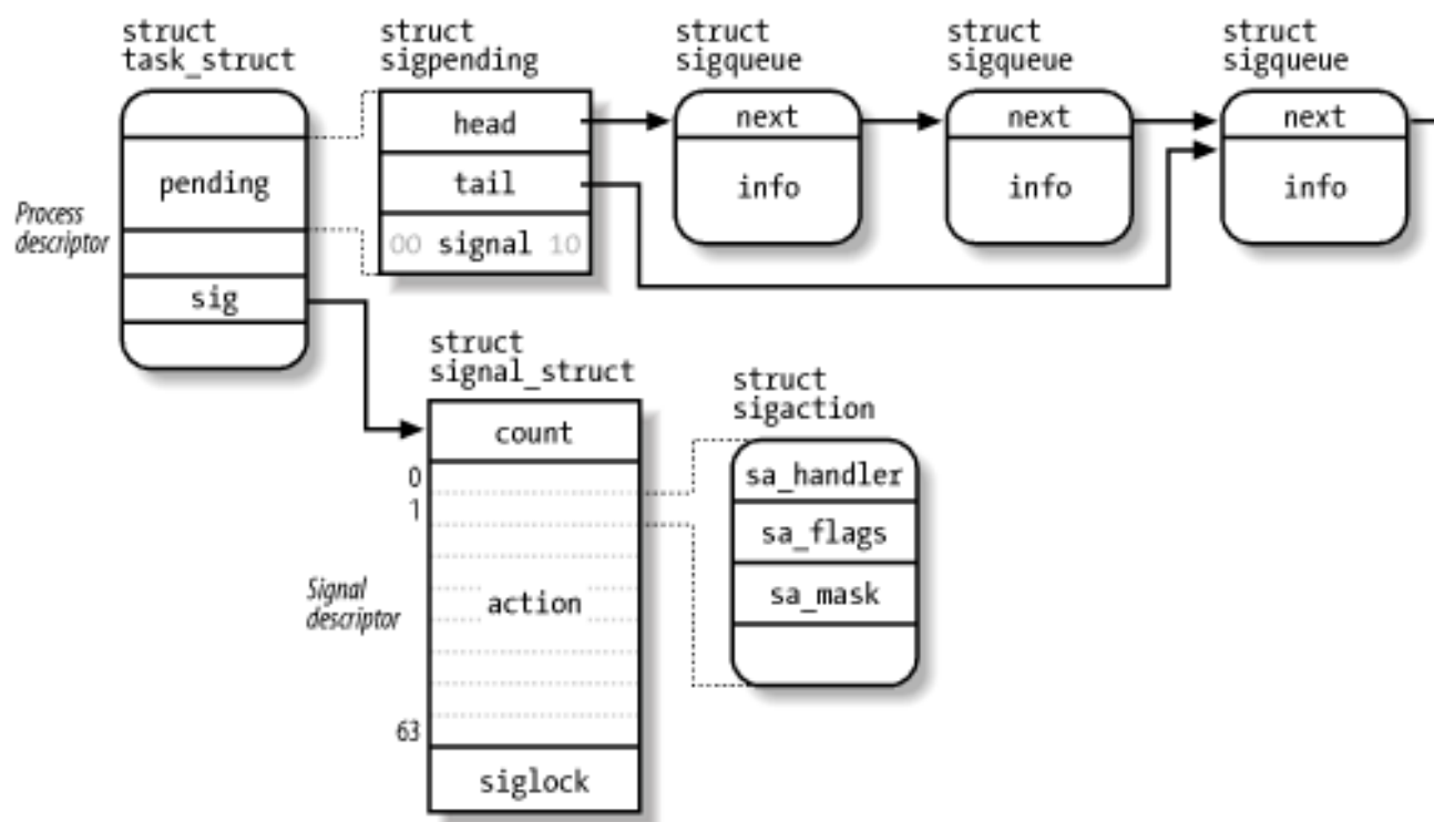
Figure 10-1. The most significant data structures related to signal handling
