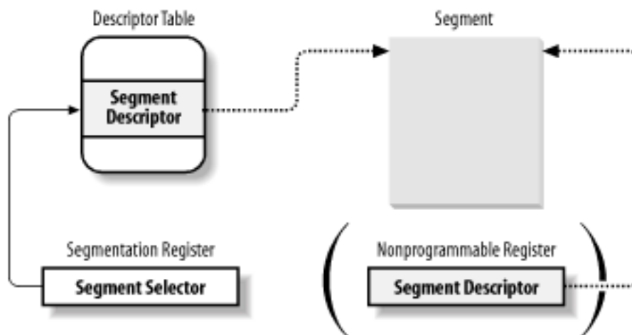
Figure 2-3. Segment Selector and Segment Descriptor
