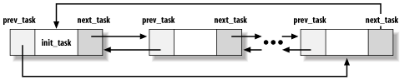
Figure 3-3. The process list
