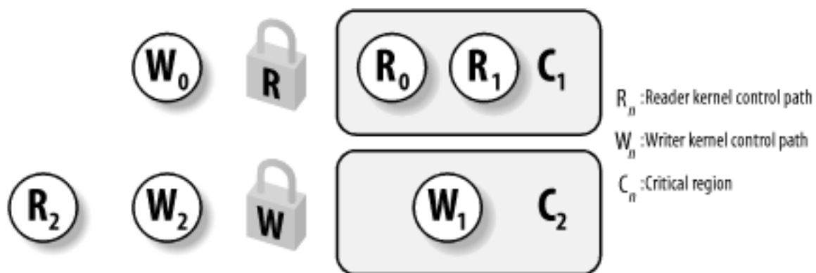
Figure 5-2. Read/write spin locks
