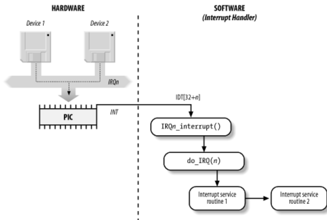
Figure 4-3. I/O interrupt handling
