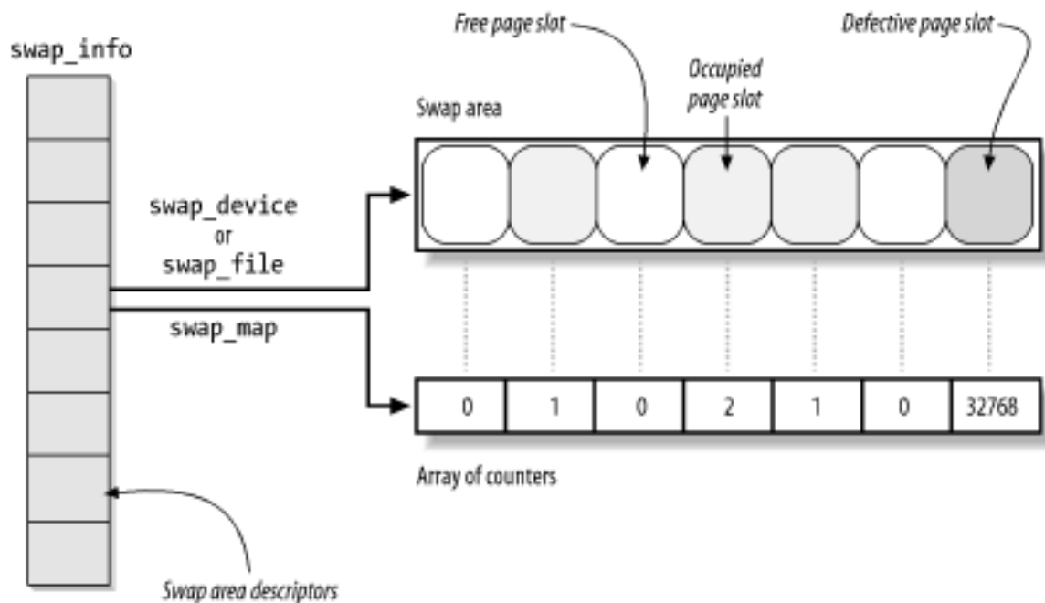
Figure 16-1. Swap area data structures
