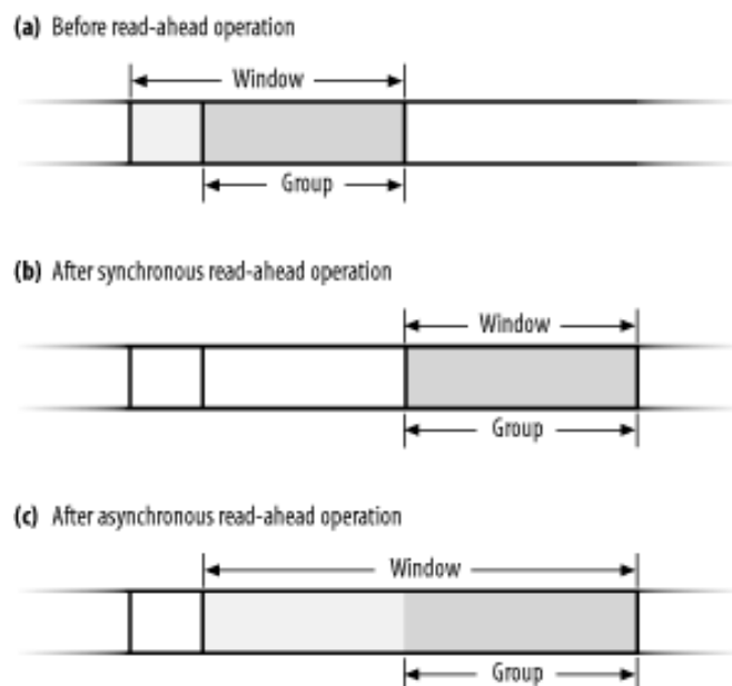
Figure 15-2. Read-ahead group and window
