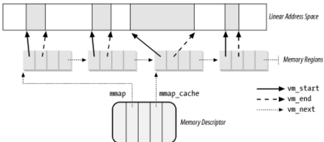
Figure 8-2. Descriptors related to the address space of a process
