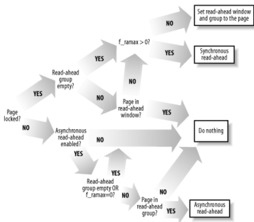
Figure 15-3. Overall scheme of the generic_file_readahead( ) function
