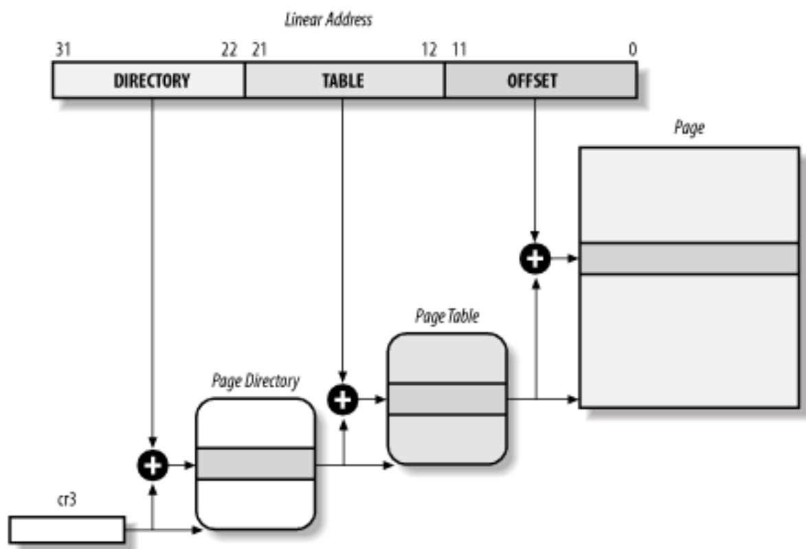
Figure 2-6. Paging by 80x86 processors
