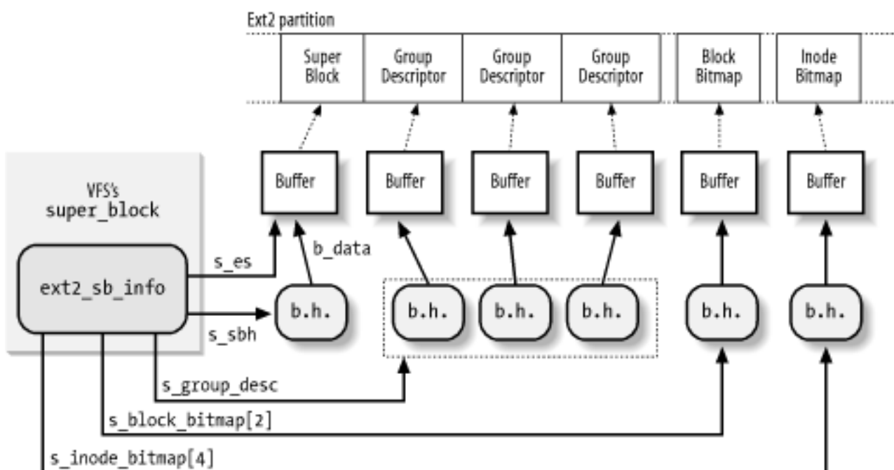
Figure 17-4. Ext2 memory data structures
