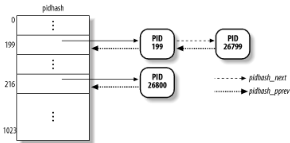
Figure 3-5. The pidhash table and chained lists
