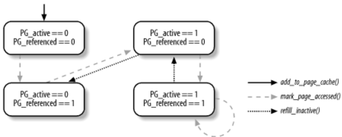
Figure 16-4. Moving pages across the LRU lists
