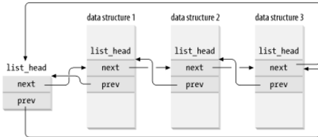
Figure 3-4. A doubly linked list built with list_head data structures
