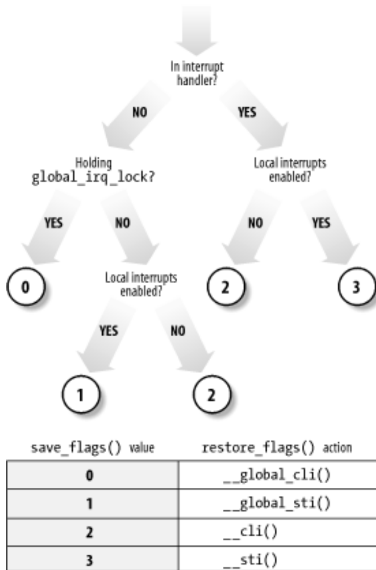
Figure 5-3. Actions performed by save_flags() and restore_flags()
