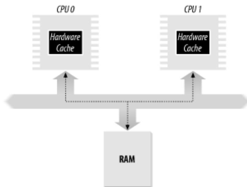
Figure 2-10. The caches in a dual processor.
