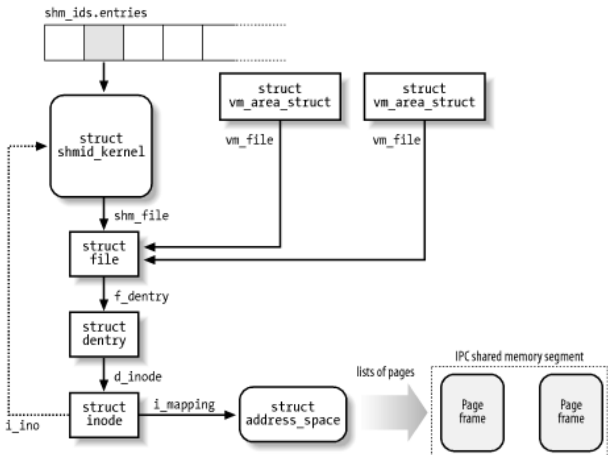
Figure 19-3. IPC shared memory data structures
