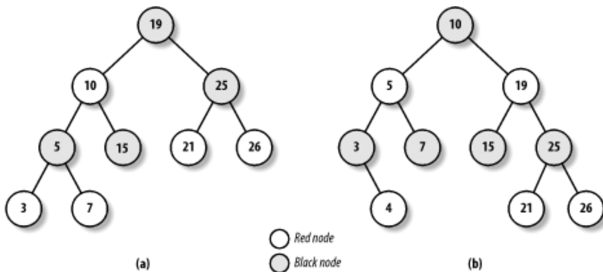
Figure 8-3. Example of red-black trees
