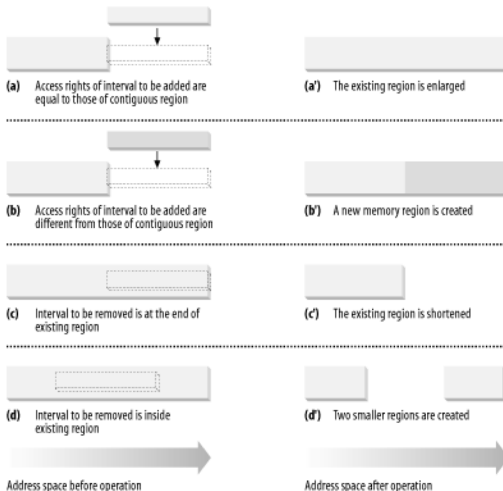
Figure 8-1. Adding or removing a linear address interval
