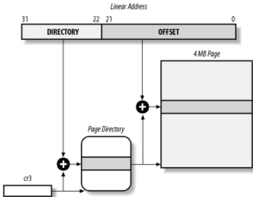
Figure 2-7. Extended paging
