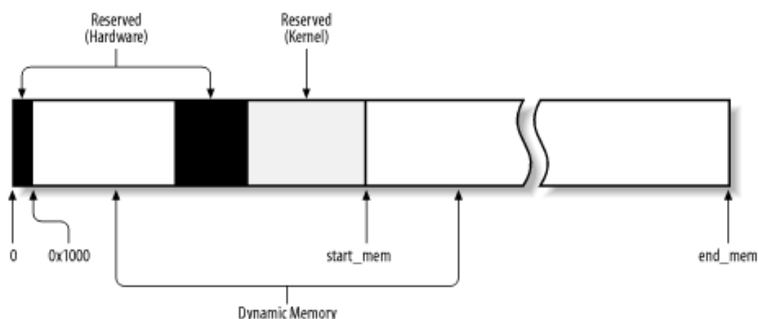
Figure 7-1. Memory layout
