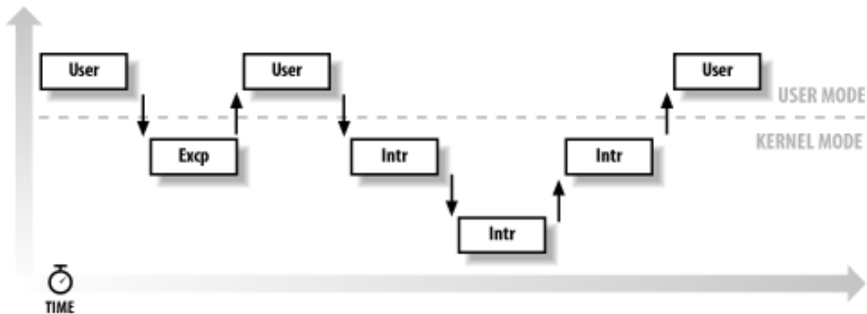
Figure 1-4. Interleaving of kernel control paths
