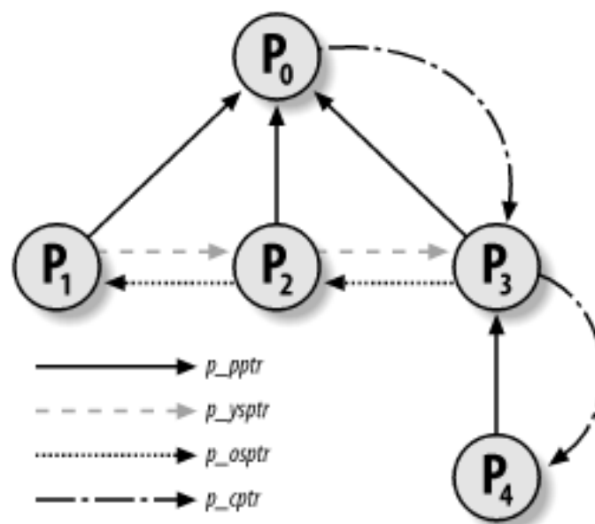
Figure 3-6. Parenthood relationships among five processes
