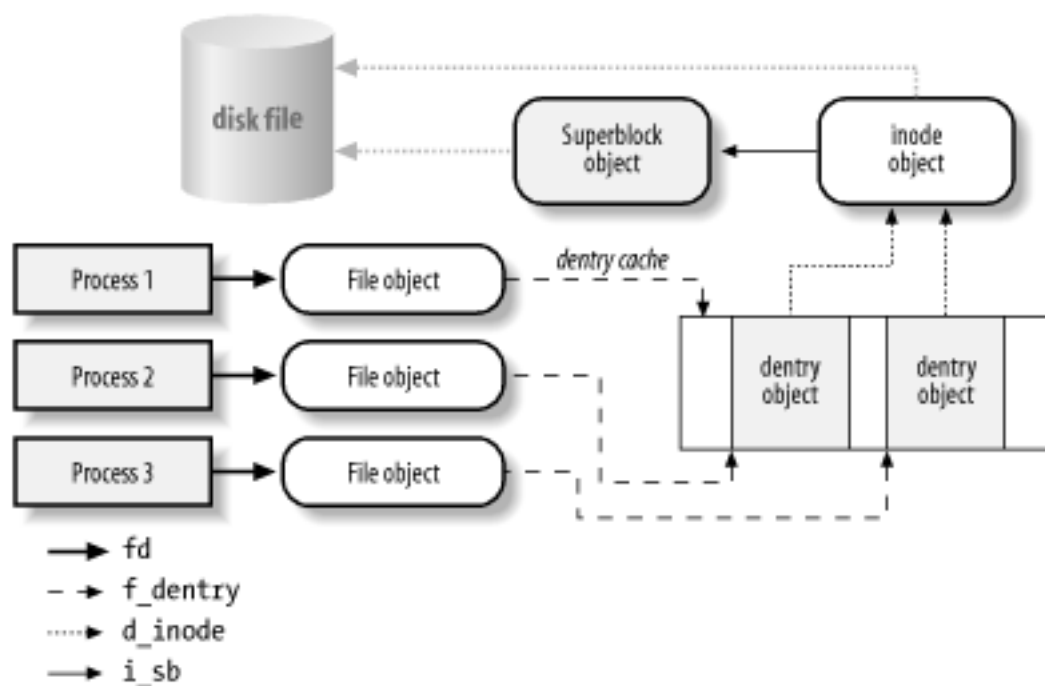
Figure 12-2. Interaction between processes and VFS objects
