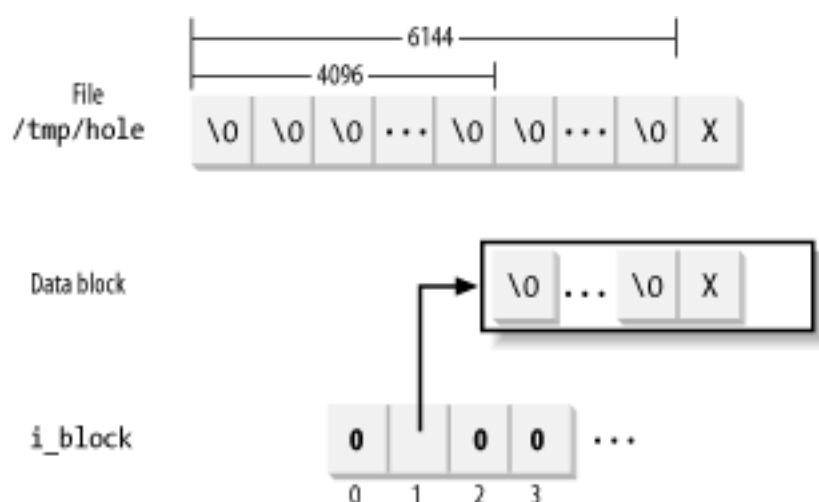
Figure 17-6. A file with an initial hole
