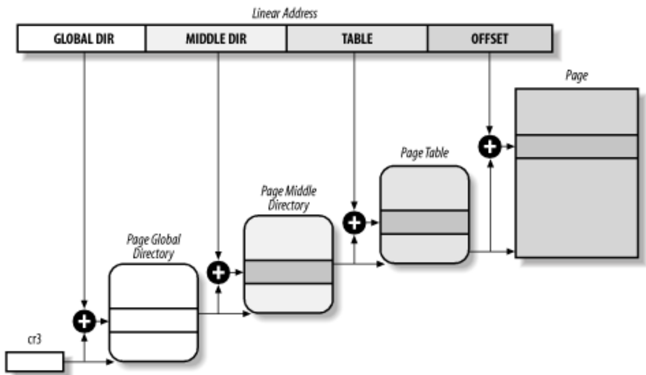
Figure 2-11. The Linux paging model
