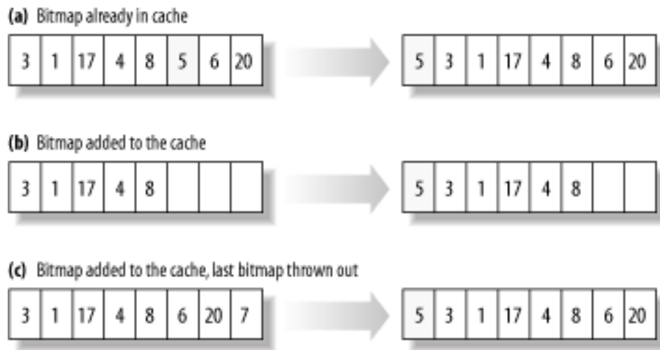
Figure 17-3. Adding a bitmap to the cache
