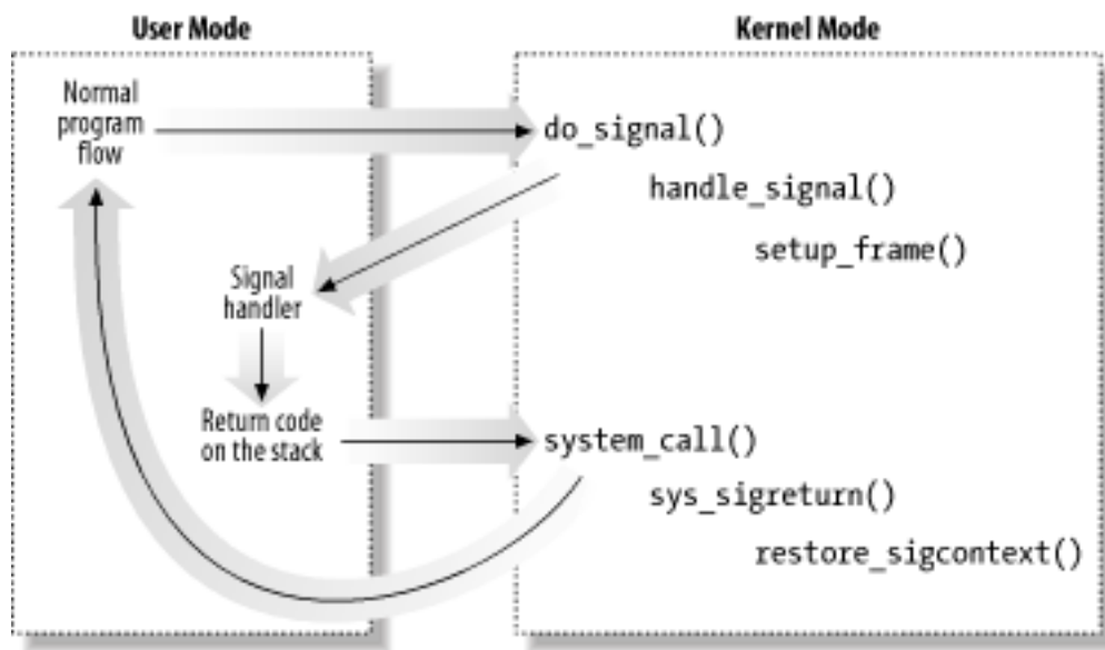
Figure 10-2. Catching a signal
