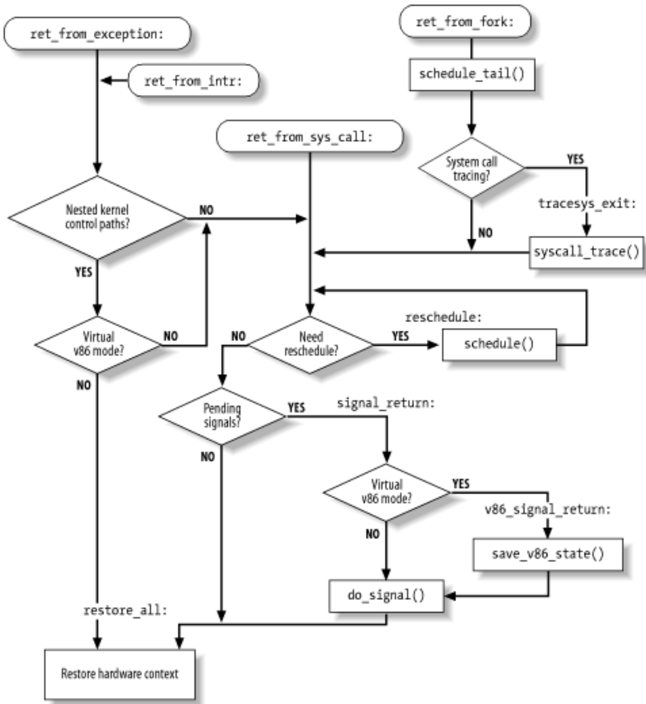
Figure 4-5. Returning from interrupts and exceptions
