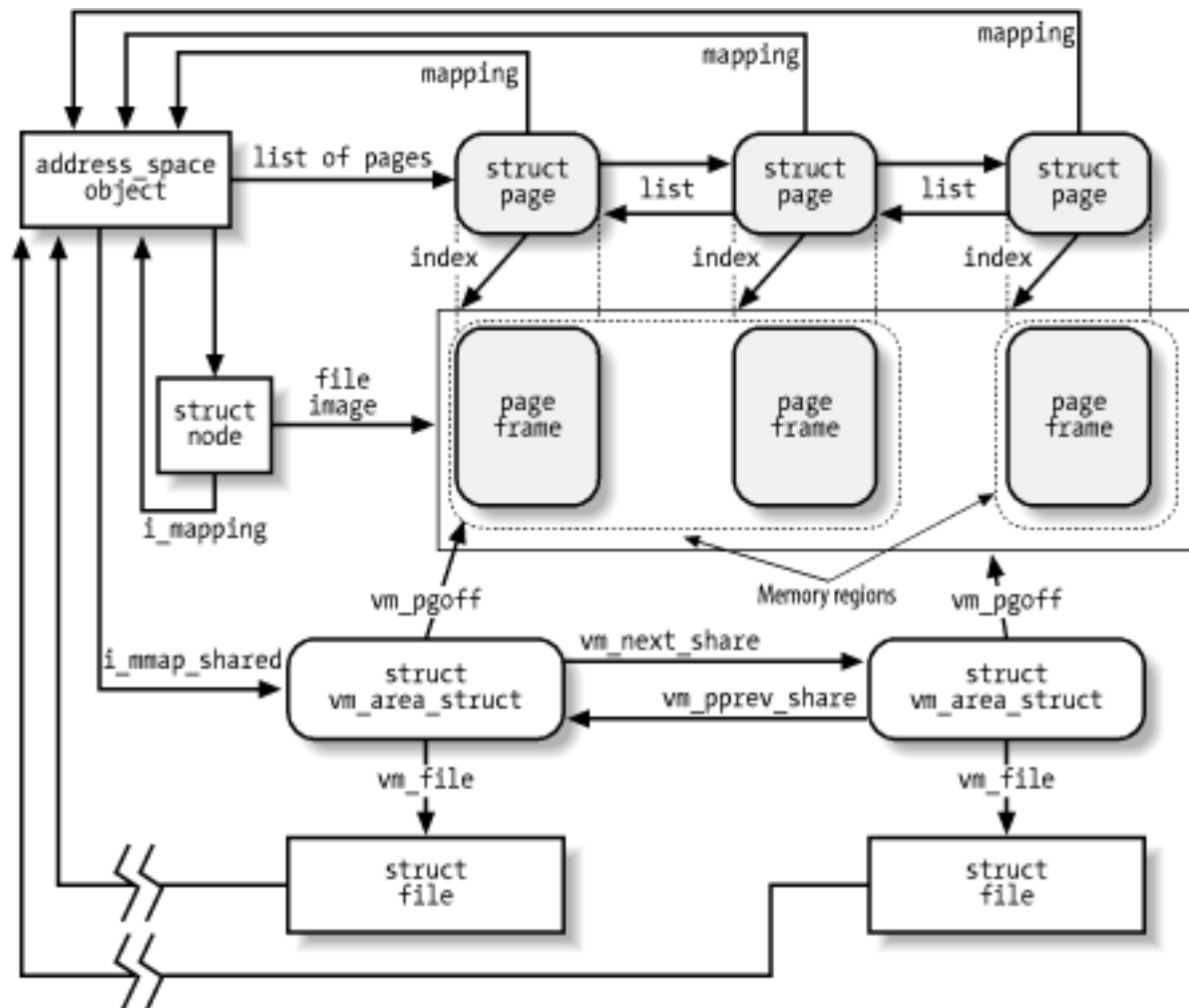
Figure 15-4. Data structures for file memory mapping
