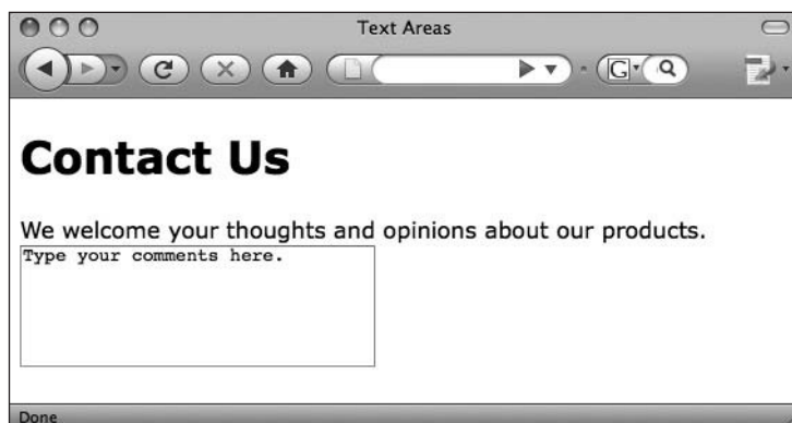
Figure 11-2 Text areas enable users to enter more than a single line of text. Any text you enter between the opening and closing textarea tags is used as the initial value of the text area.
