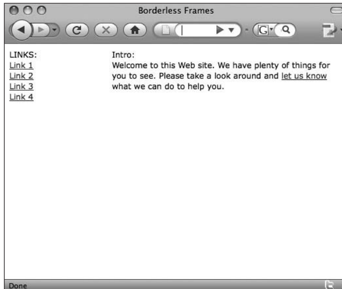
Figure 10-3 The best way to turn off the space completely between the frames is to set both the border and frameborder attributes to 0.
