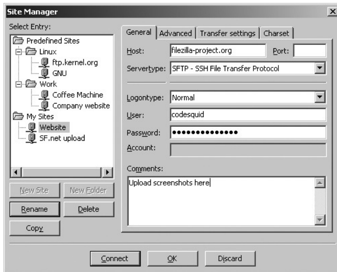
Figure 17-3 Use FileZilla’s Site Manager to store usernames and passwords for frequently accessed FTP sites.
