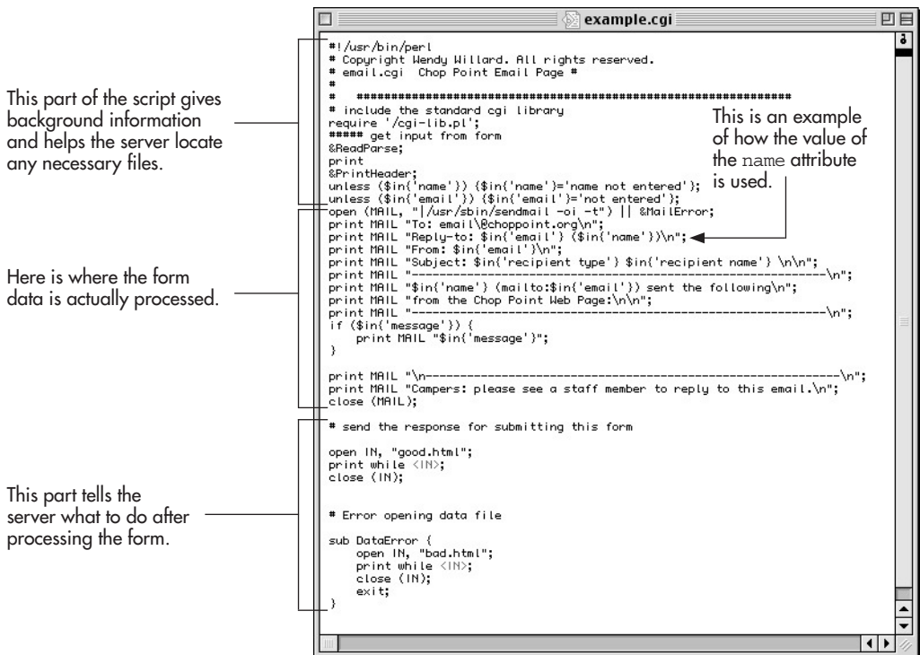
Figure 11-6 This CGI script, written in Perl, was used to process a form that lets parents and friends e-mail kids at camp.
