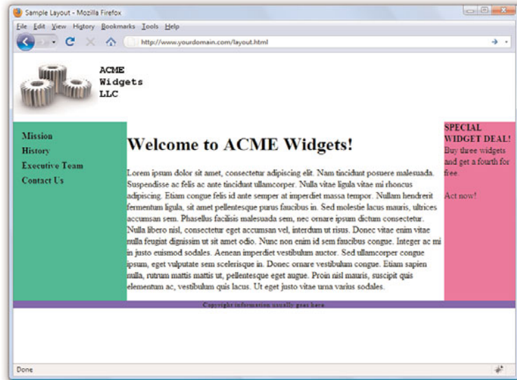
LISTING 12.2 Basic Fixed/Liquid Hybrid Layout Structure (with Content)
