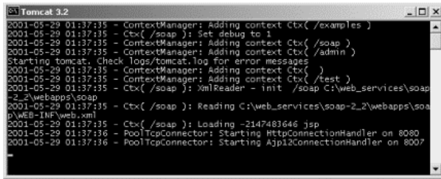
Figure 4-1. Starting Tomcat
