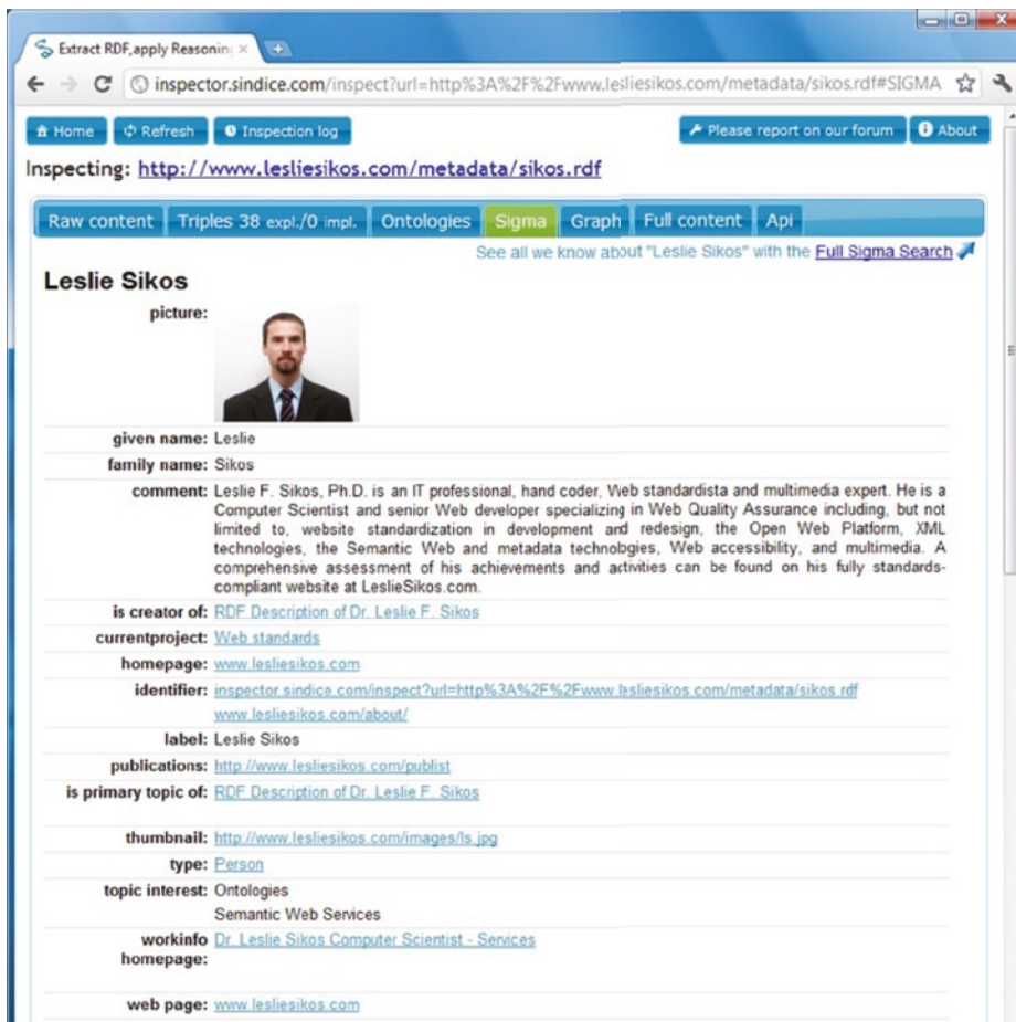
Figure 14-16. A personal description extracted from RDF and displayed in a visually appealing manner
